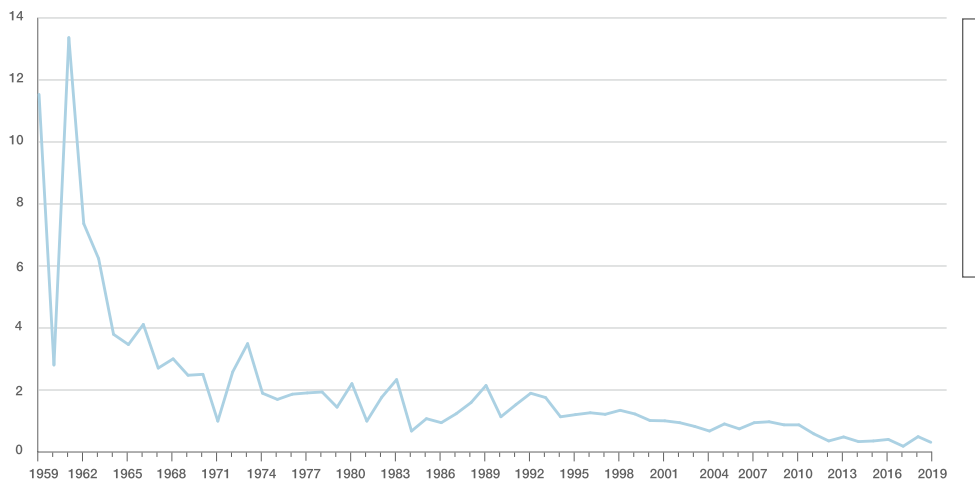
Yearly hull loss rate per million flights
