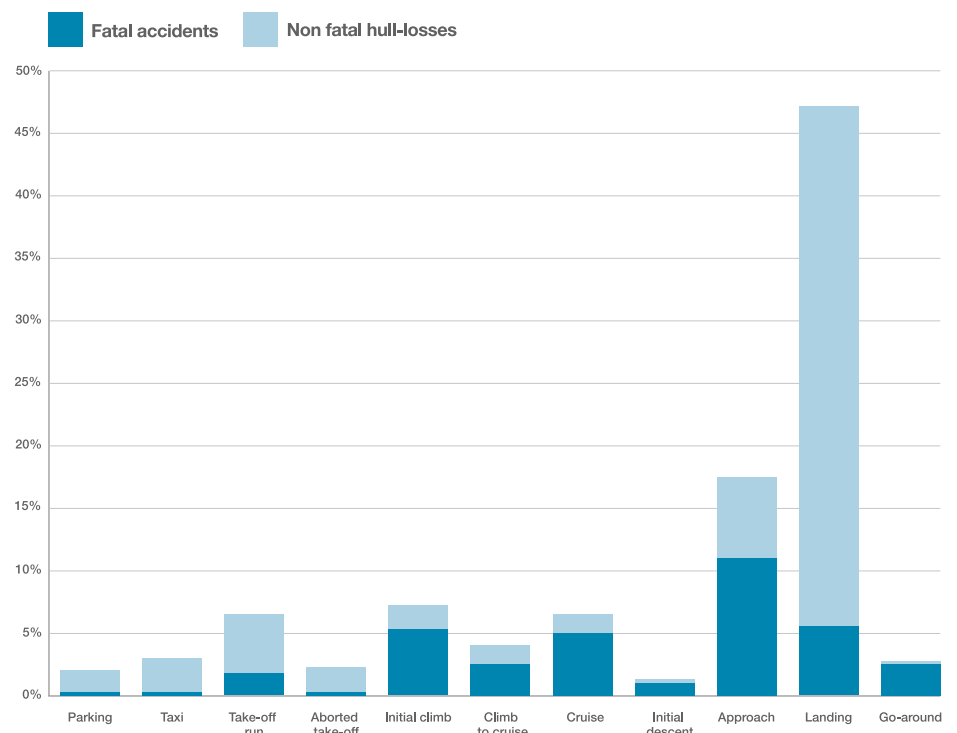
Accidents per flight phase distribution 1999-2019
