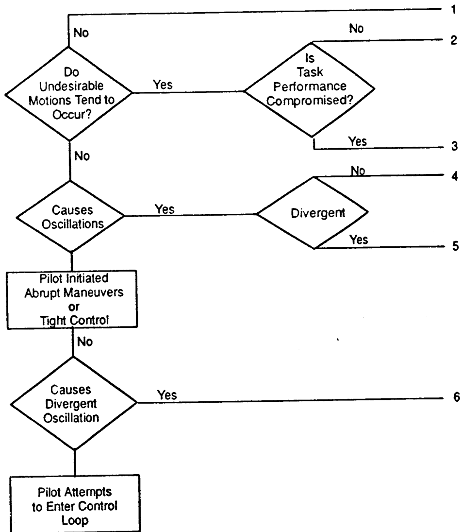
FIGURE 12. PIO tendency classification from AFWAL-TR-81-3118.
