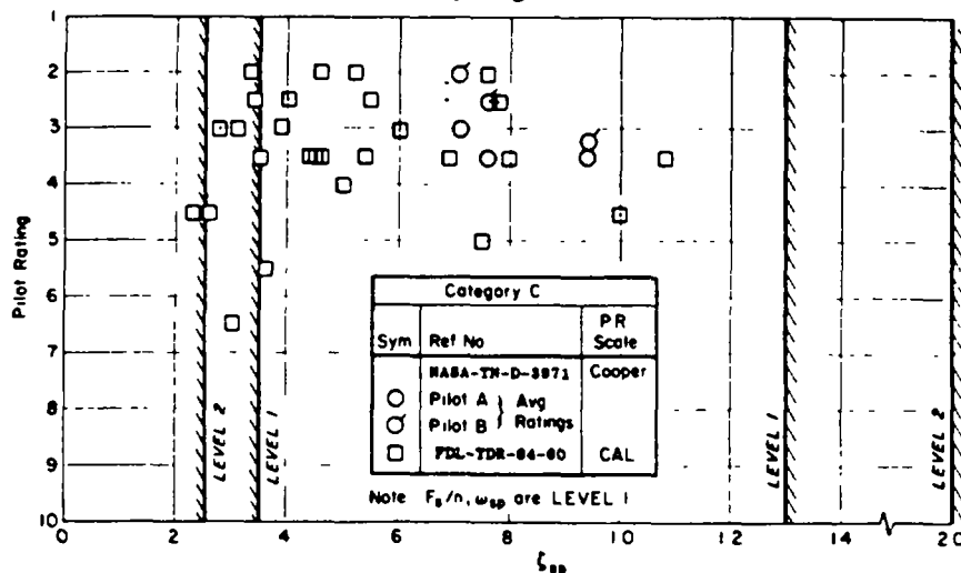
FIGURE 38. Comparison of pilot ratings with Category C short-period damping requirements.
