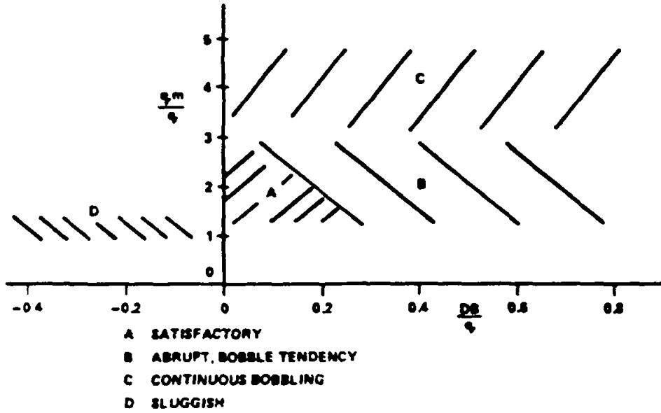
FIGURE 80. Precision tracking: q \sim \theta trends.
