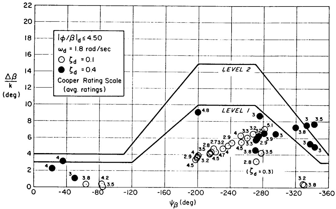
FIGURE 241. Category C configurations of Princeton Univ Rpt 727 ( \Delta\beta/k , \psi_\beta from AFFDL-TR-72-41).
