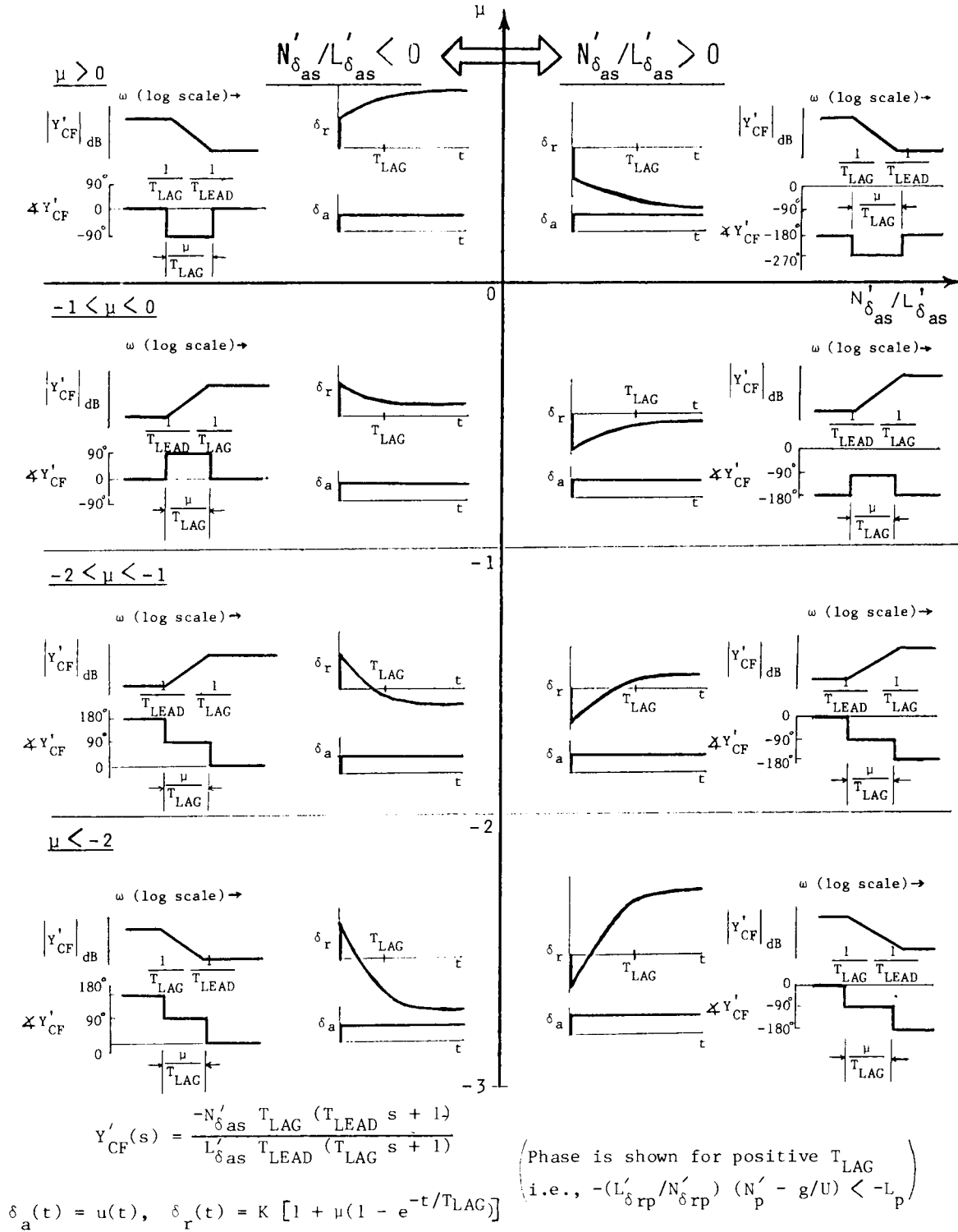
FIGURE 249. Bode asymptotes and time response of crossfeed.
