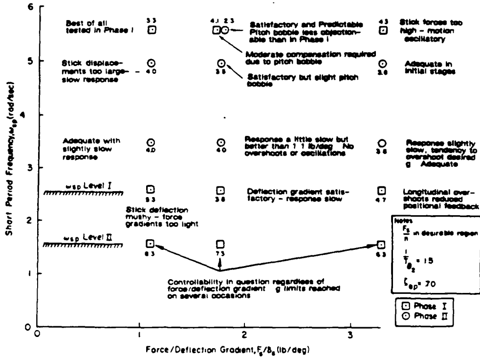
FIGURE 122. Average pilot ratings for gross acquisition task.
