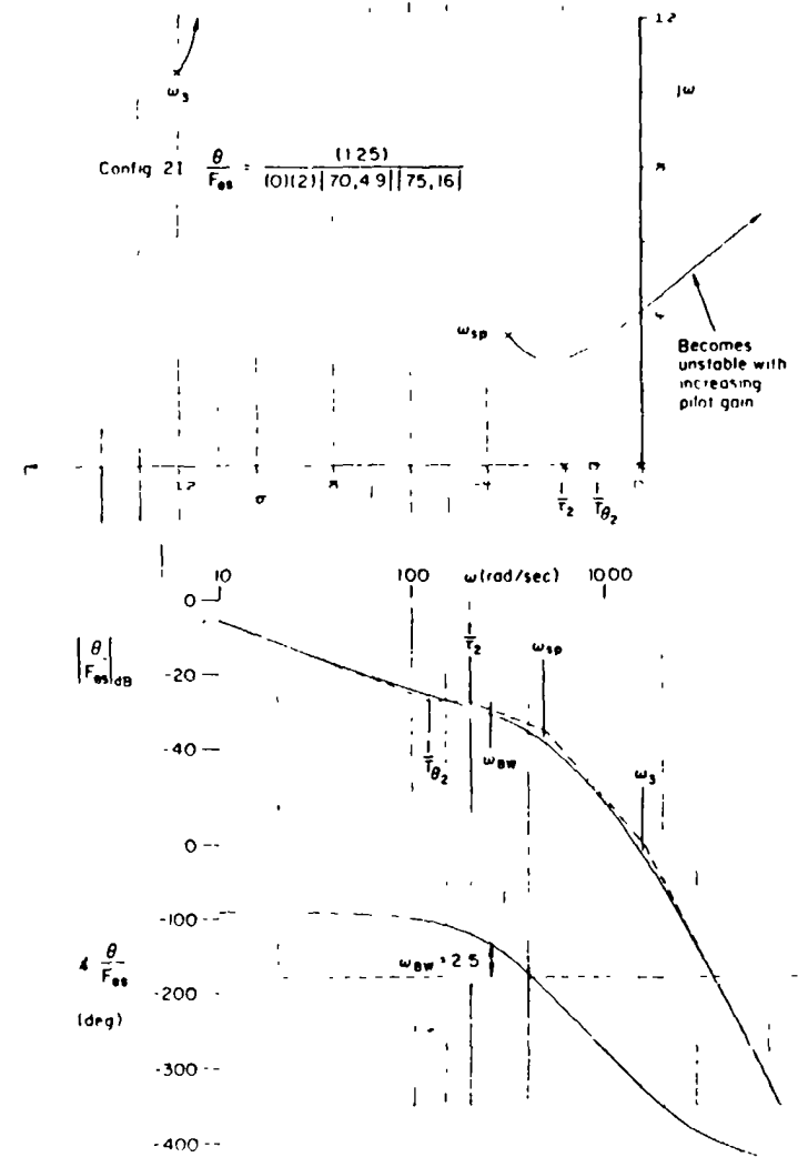
FIGURE 61b. Level 3 system of Neal-Smith (2I) \omega_{BW} = 2.5 mean PR = 8.0.
