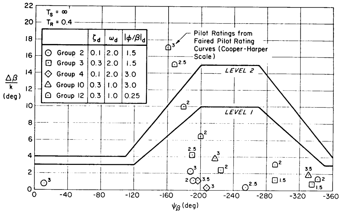
FIGURE 242. \Delta\beta_{\max}/k versus \psi_\beta for configurations that meet Level 1 p_{\text{osc}}/p_{\text{av}} , \zeta_d , and \zeta_d\omega_d criteria (from AFFDL-TR-70-145).
