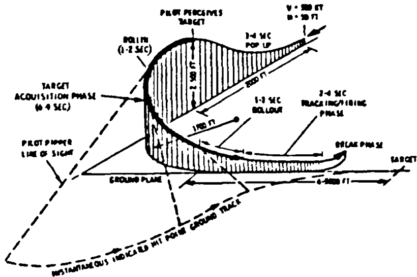
FIGURE 4. Ground attack maneuver scenario.
