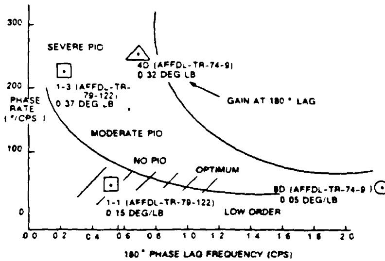
FIGURE 77. Trends of high order phase rate.
