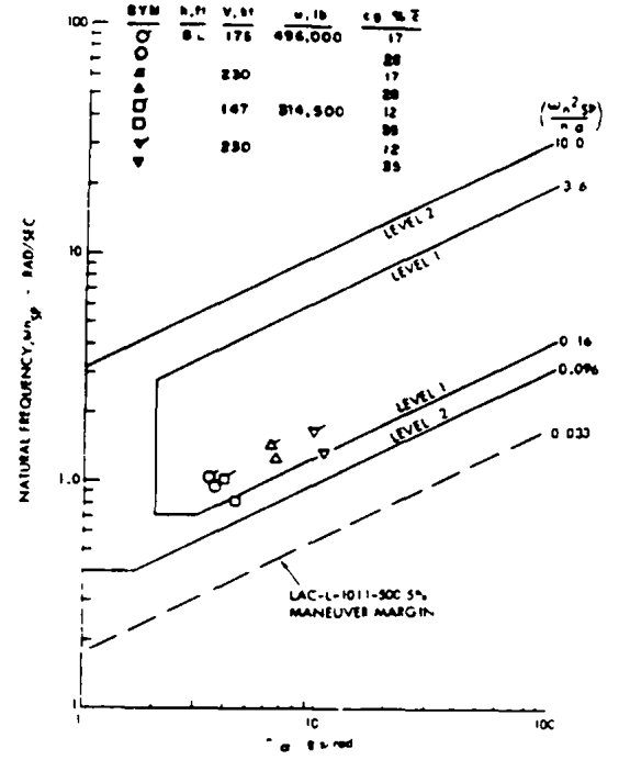
b) L-1011 takeoff configuration.
