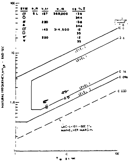
c) L-1011 power approach configuration.
