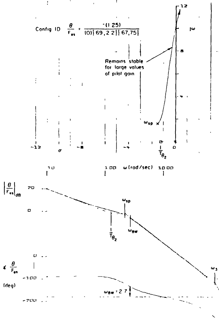
FIGURE 61a. Level 1/2 system of Neal-Smith (1D): \omega_{BW} = 2.7 rad/sec, mean PR = 4.1.
