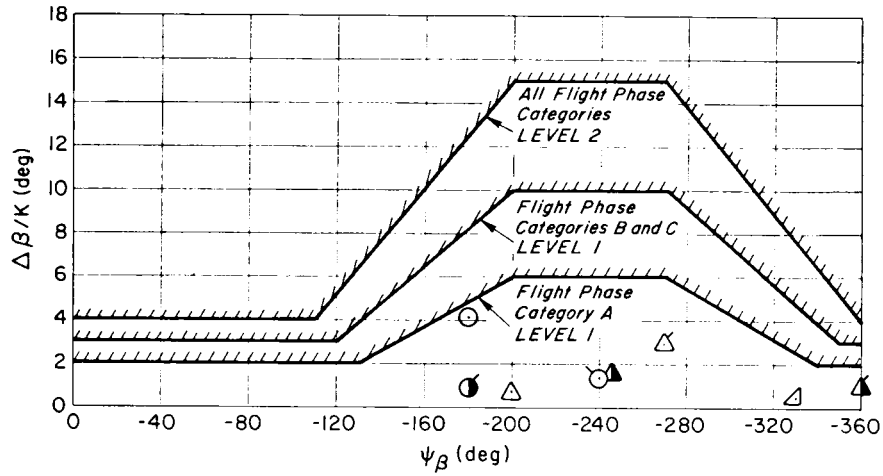
a) Small Inputs
