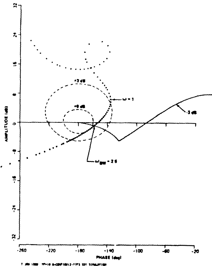
FIGURE 70. Amplitude-phase plot for configuration 12 (aft; c.g. - unstable).
