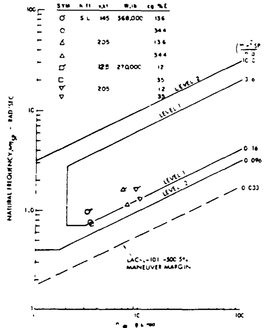
d) L-1011 landing configuration.
