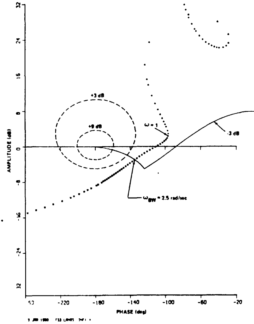
FIGURE 72. Amplitude-phase plot for configuration 6-2.
