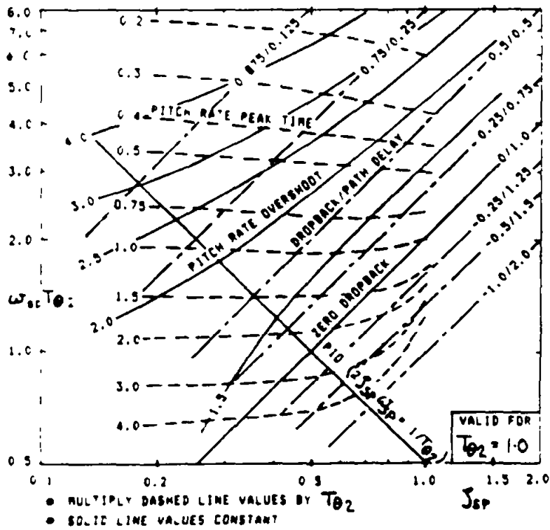
FIGURE 81. New short-period thumbprint (from ICAS-86-5.3.4).
