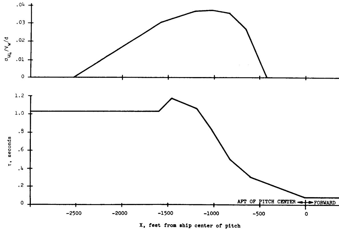
FIGURE 269. u-component burble time constant and variance.
