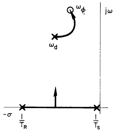
c) Moderate \zeta_d ; Zero Above Pole
