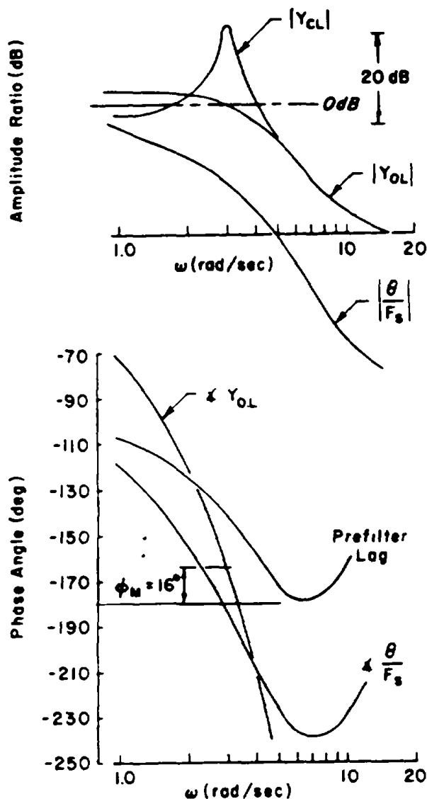
FIGURE 92. YF-17 pitch attitude dynamics (AFFDL-TR-77-57).
