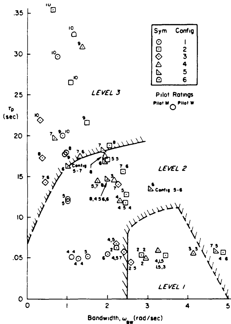
FIGURE 65. Correlation of pilot ratings with \omega_{BW} and \tau_p for approach and landing (AFFDL-TR-122).
