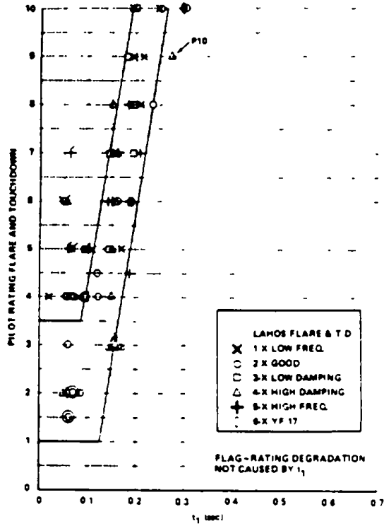
FIGURE 52. Pilot rating correlation with effective time delay (AFFDL-TR-78-122 data).
