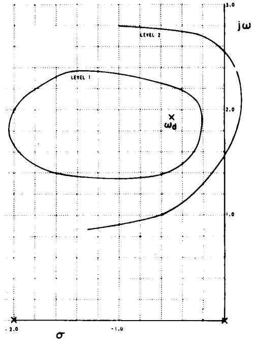
b) \omega_d = 2 \text{ rad/sec} ; \zeta_d = 0.25
