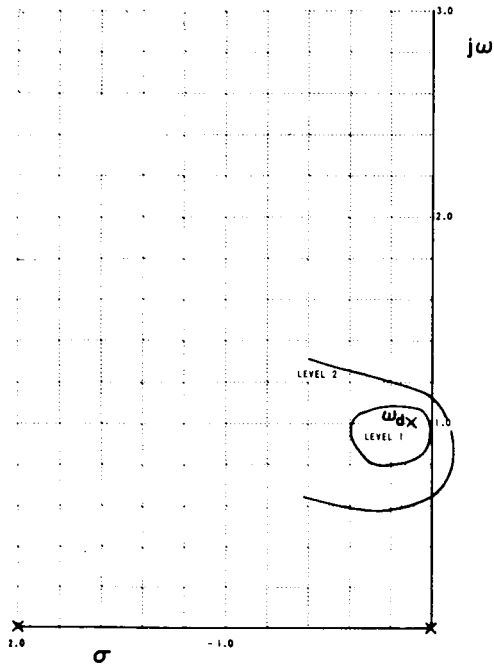
c) \omega_d = 1.0 \text{ rad/sec} ; \zeta_d = 0.1
