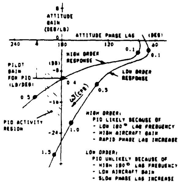
FIGURE 76. High and low order frequency response.
