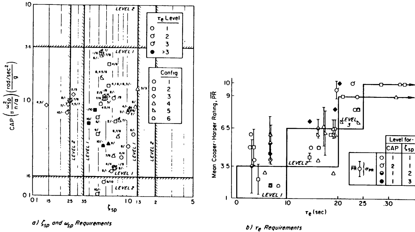
FIGURE 45. Comparison of LOES dynamics with short-period requirements; Category C, LAHOS (AFFDL-TR-78-122) configurations, MCAIR ("Equivalent Systems Approach for Flying Qualities Specification").
