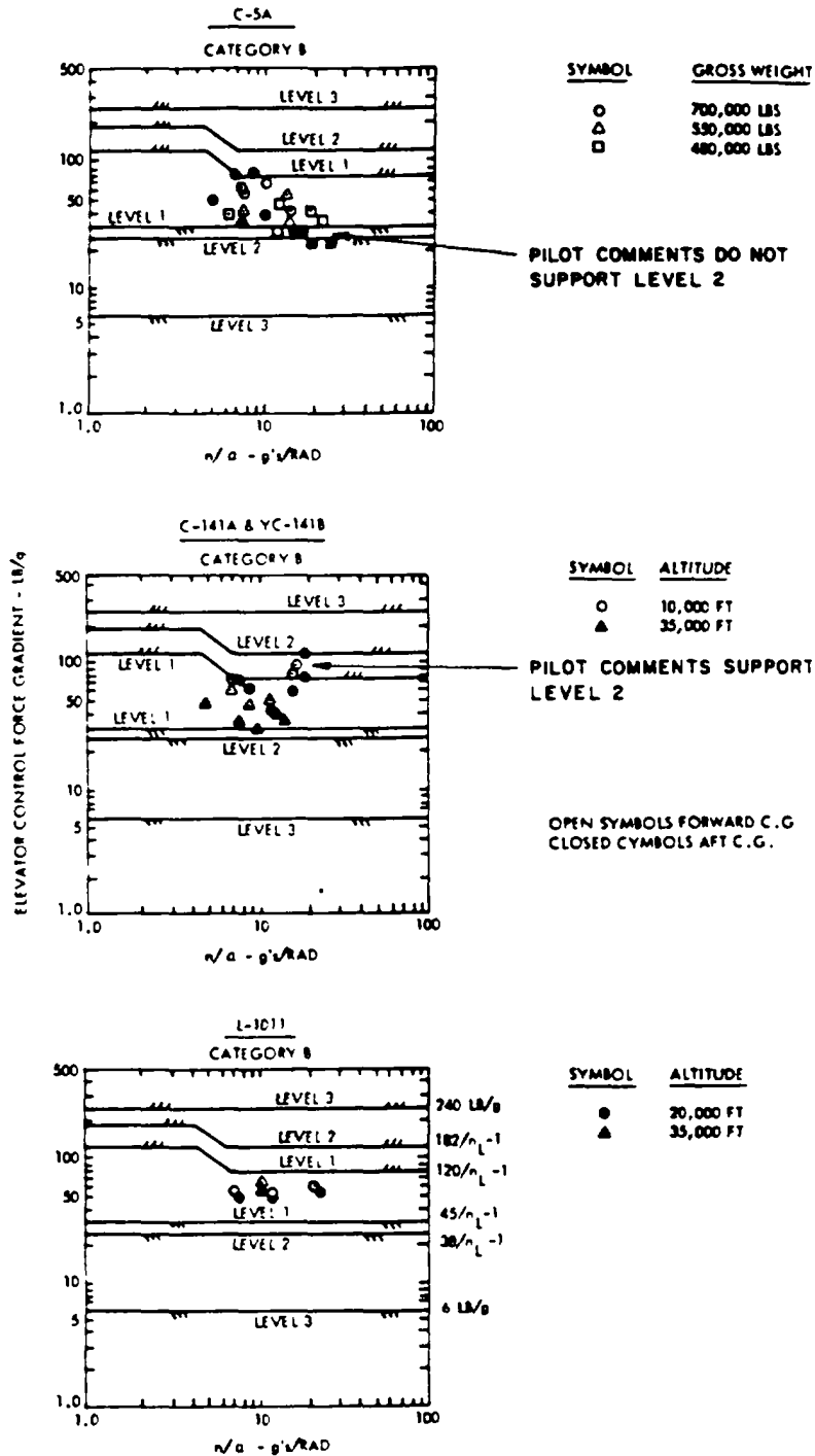
FIGURE 111. Elevator control force gradients for transport aircraft (from AFFDL-TR-78-171).
