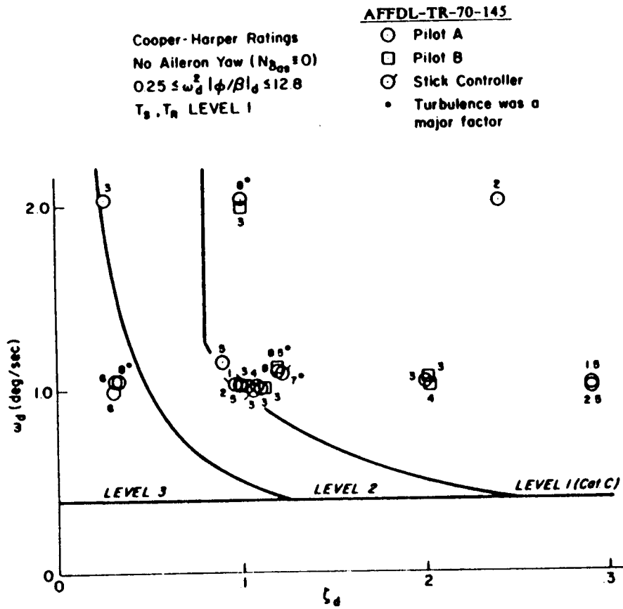
FIGURE 220. Dutch roll data from In-flight simulation of Class II-L airplanes in landing approach (T-33; AFFDL-TR-70-145).
