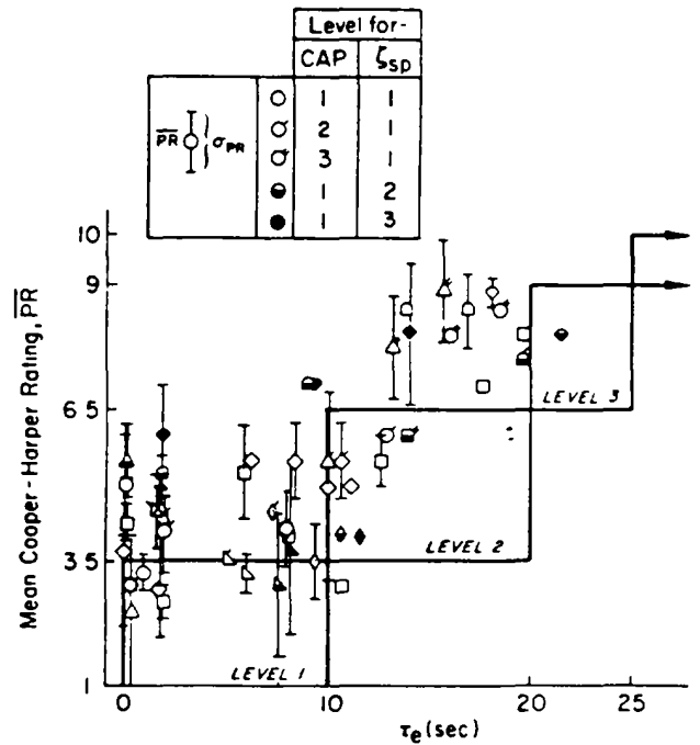
b) \tau_e Requirements
