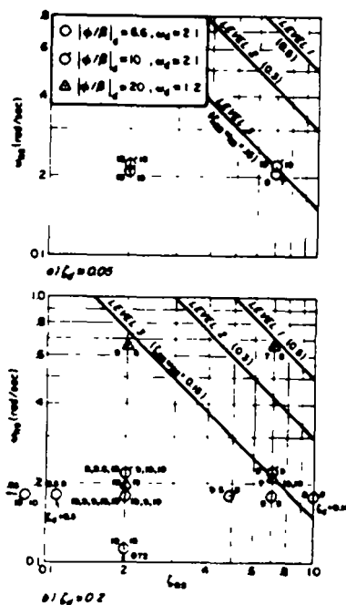
FIGURE 154. Pilot ratings for ground simulation of AFFDL-TR-65-39 [(\omega_\phi/\omega_d)^2 = 0.64 - 1.10] .
