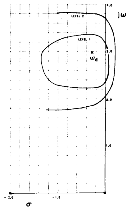
d) \omega_d = 3.0 \text{ rad/sec} ; \zeta_d = 0.1
