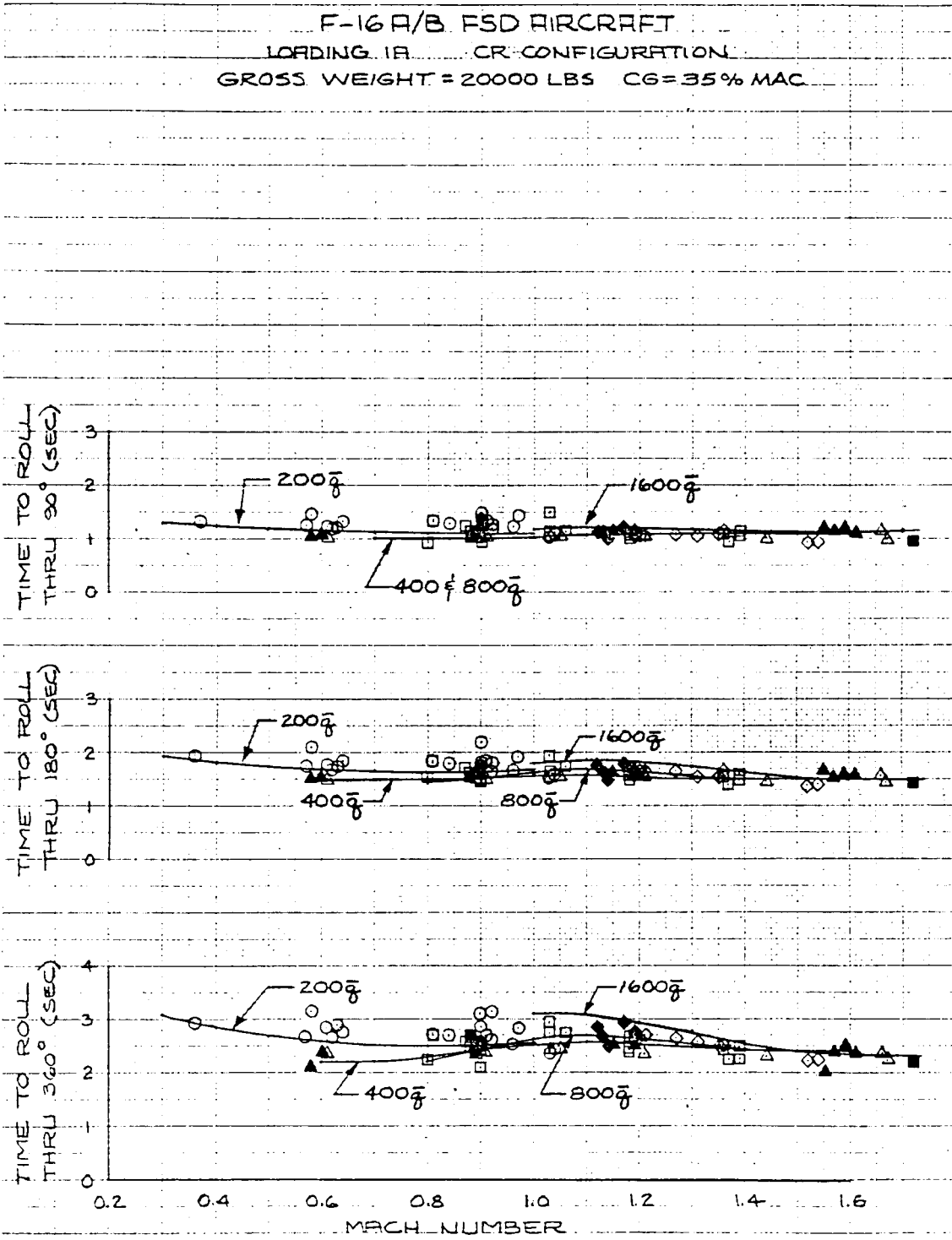
FIGURE 187. Roll performance summary (from AFFTC-TR-79-10)-Continued.
