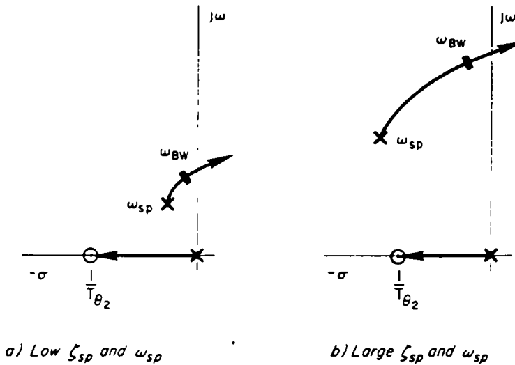
FIGURE 58. Simplified pilot-vehicle closure for pitch control.
