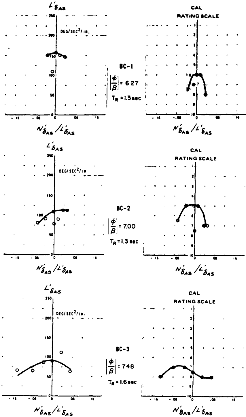
FIGURE 137. Pilot ratings and optimum aileron sensitivity (Medium \left| \frac{\phi}{\beta} \right|_d , Long T_R ) (from AFFDL-TR-67-98).
