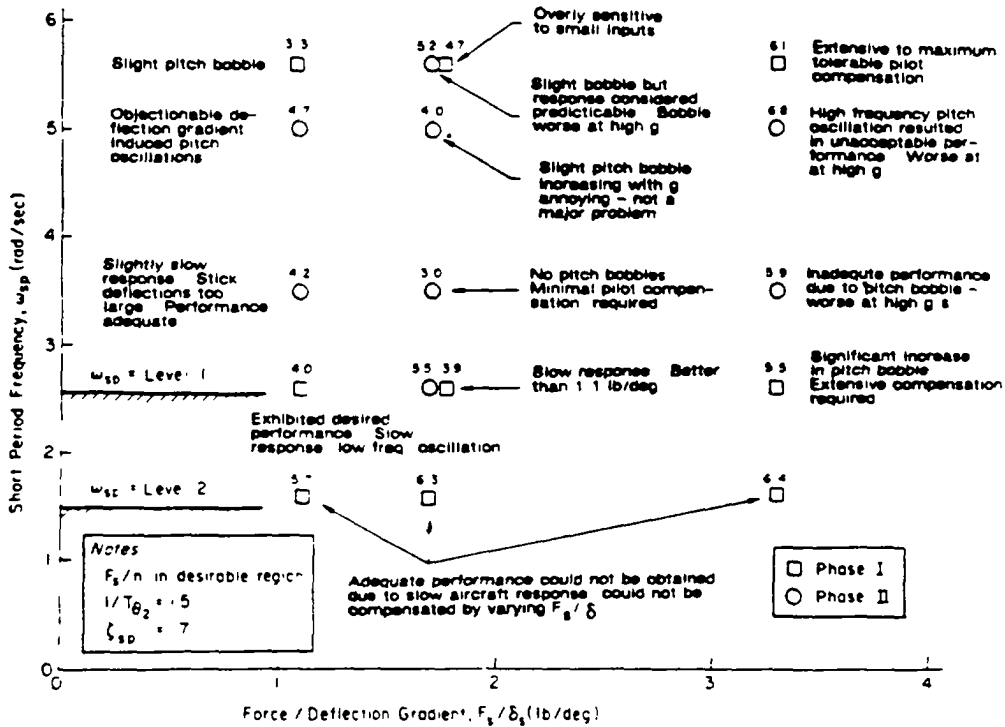
FIGURE 123. Average pilot ratings for fine tracking tasks.
