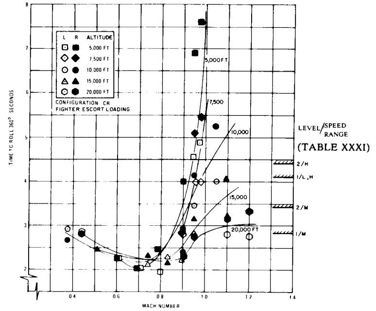
FIGURE 184. Time to roll 360° versus mach for F/A-18A (Navy Rpt No. SA-14R-81).
