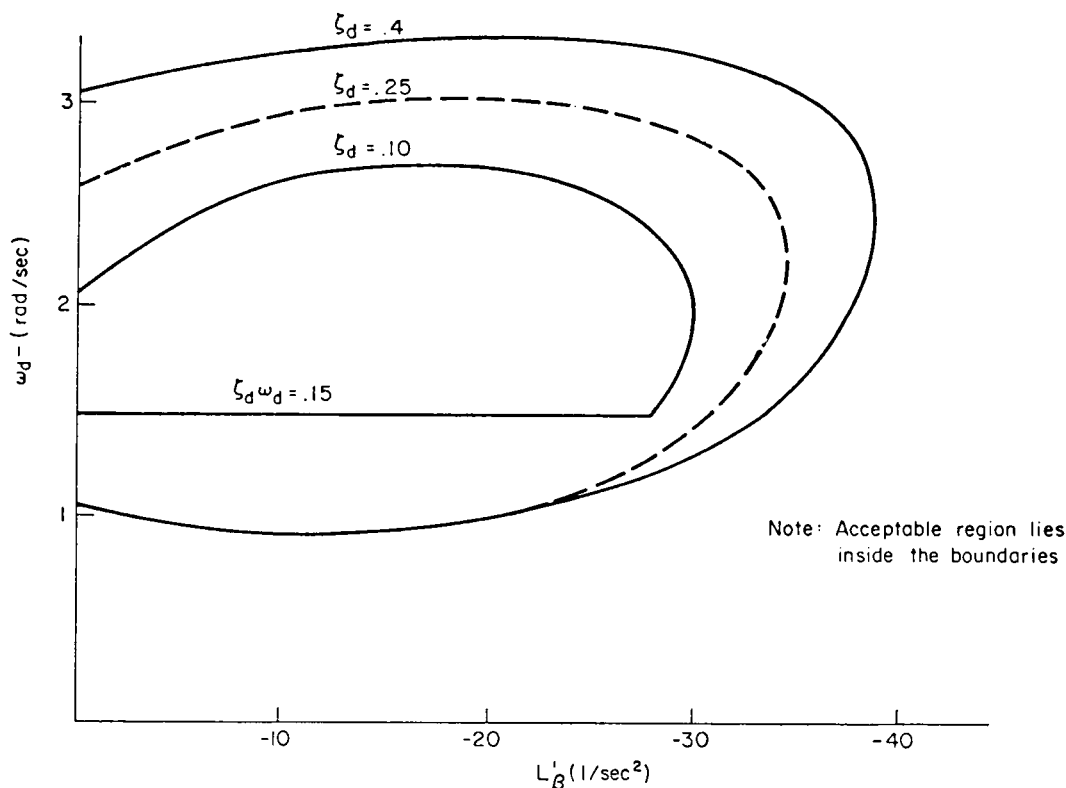
FIGURE 248. Pilot rating boundaries for acceptable roll control in turbulence with |\dot{r}_o/\dot{p}_o| \leq 0.03 (from Princeton Univ Rpt 797).
