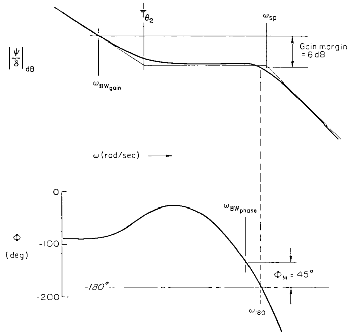
FIGURE 229. Definition of bandwidth frequency.
