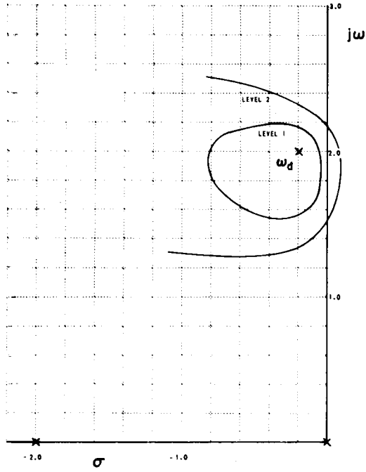
a) \omega_d = 2 \text{ rad/sec} ; \zeta_d = 0.1
