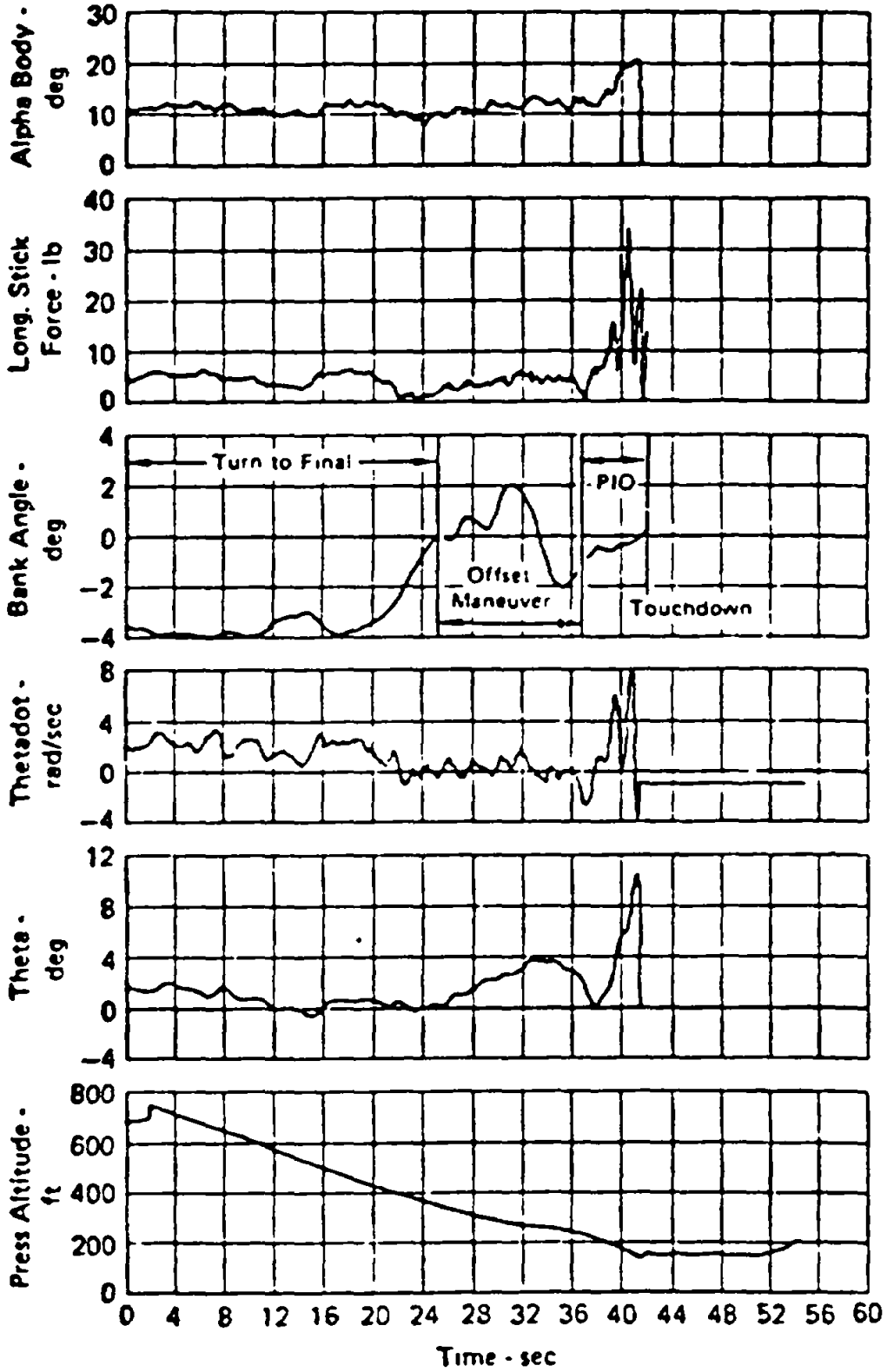
FIGURE 91. Pilot-induced oscillation at touchdown.
