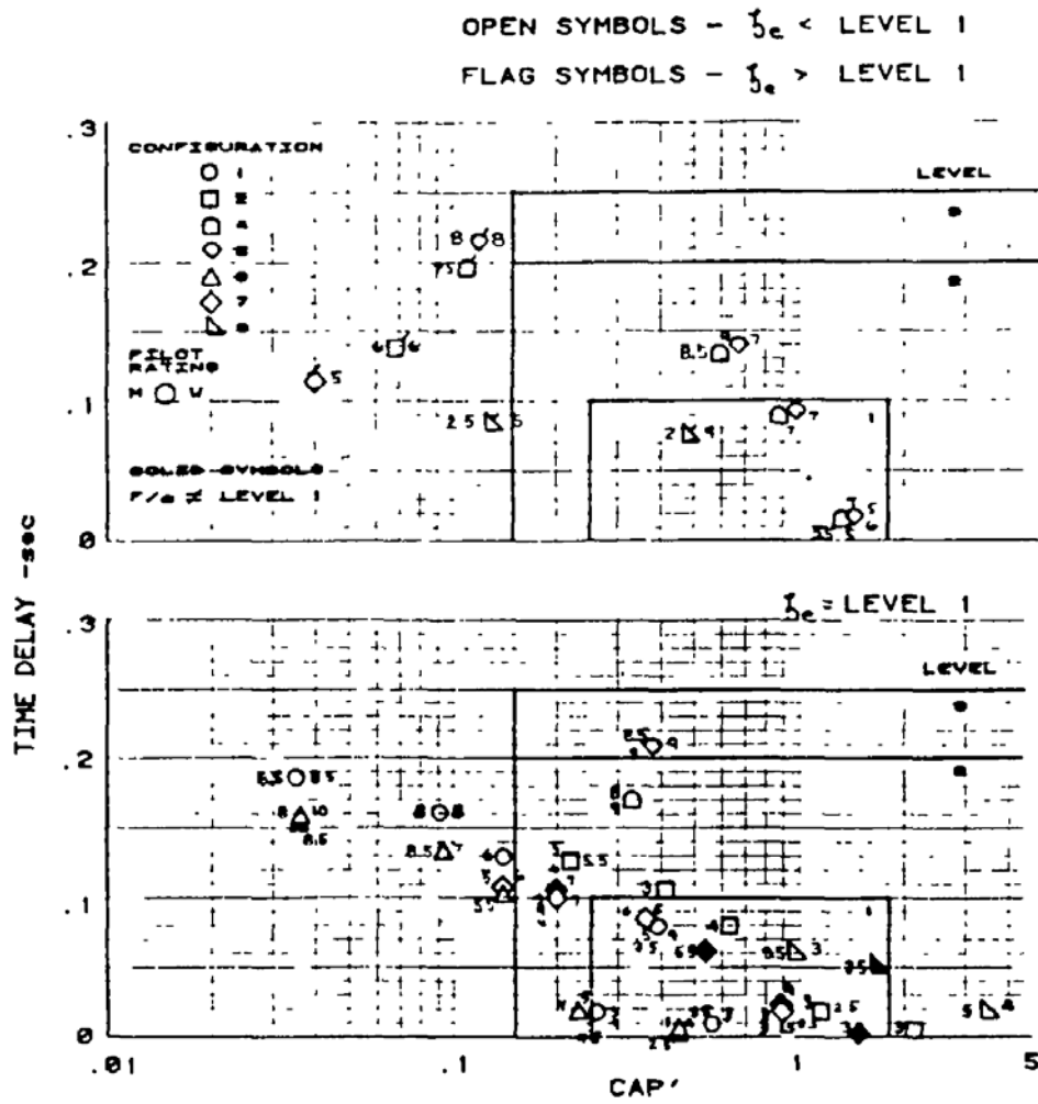
FIGURE 22. Time delay versus CAP' - Neal-Smith data
