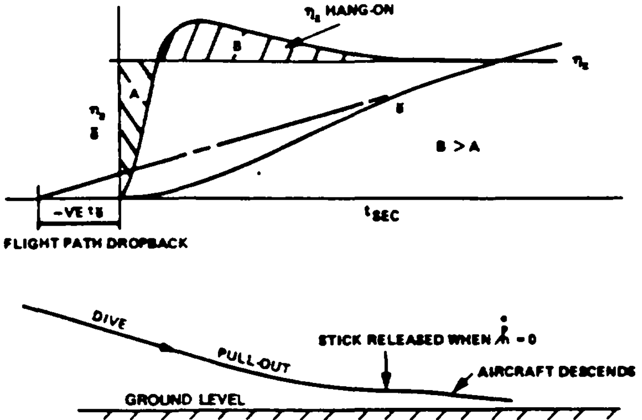
FIGURE 78. Flight path - attitude relationships.
