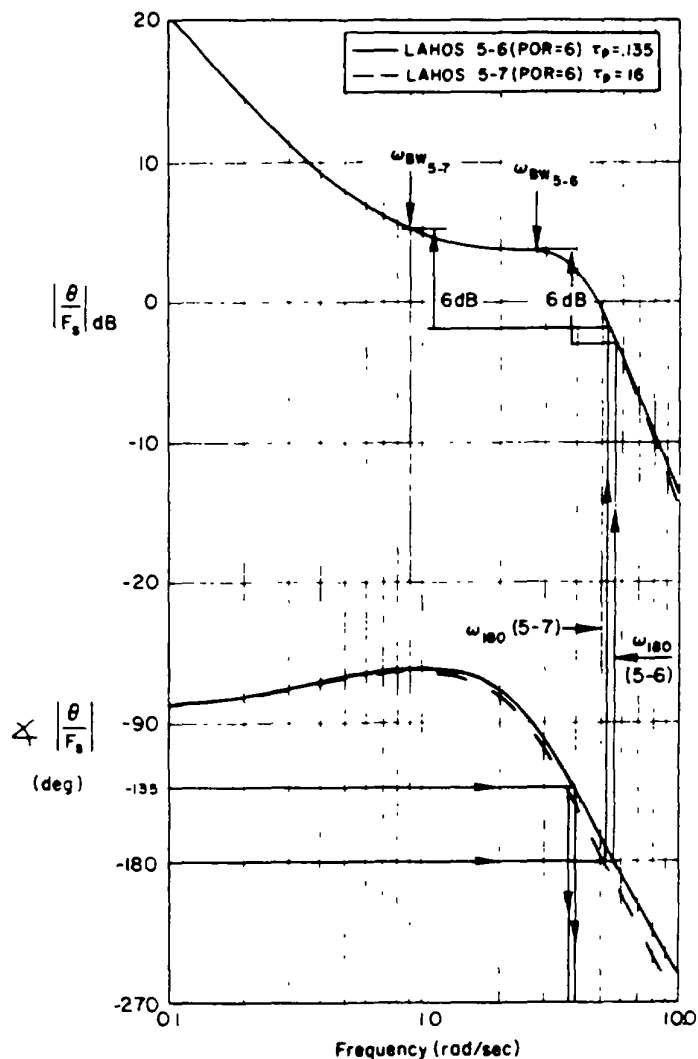
FIGURE 63. Large difference in bandwidth due to shelf in amplitude plot with moderate values of \tau_p (configurations of AFFDL-TR-78-122).
