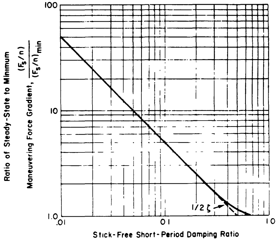
FIGURE 114. The ratio (F_s/n)/(F_s/n)_{\min} vs. \zeta_{sp} .
