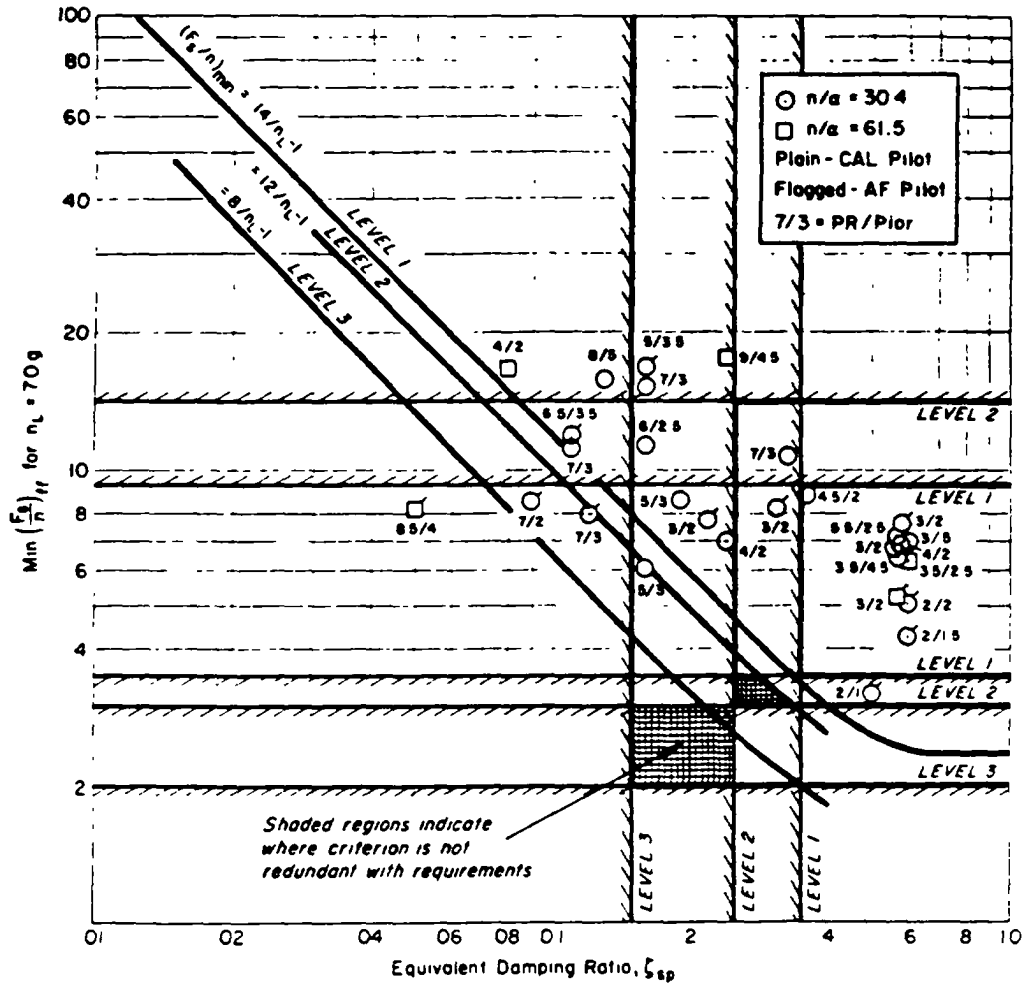
FIGURE 116. Comparison of (F_s/n)_{\min} boundaries with (F_s/n)_{SS} and \zeta_{sp} for cases where \omega_{sp} \ll \omega_{cs} (AFFDL-TR-66-163).
