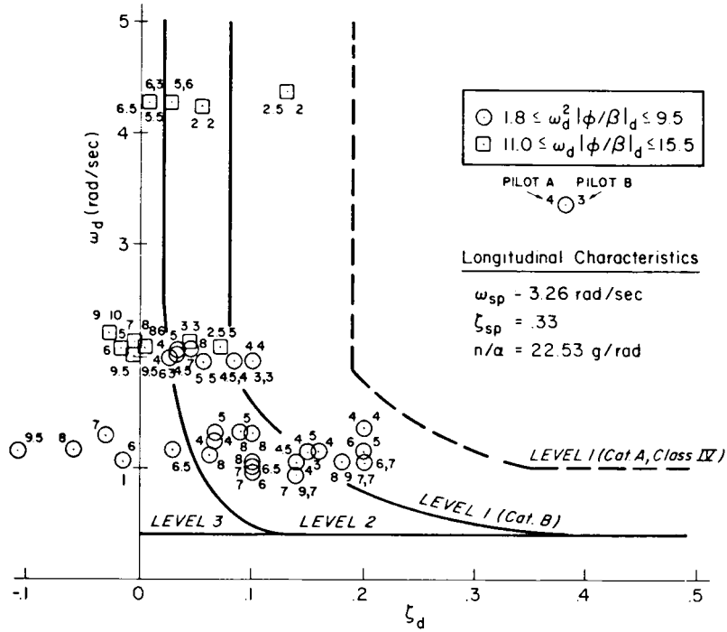
a) \omega_d^2 |\phi/\beta|_d < 20 (rad/sec)^2
