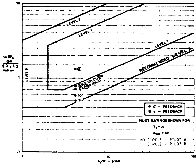
c) Short aft tail, x_{mp} = 50 ft
