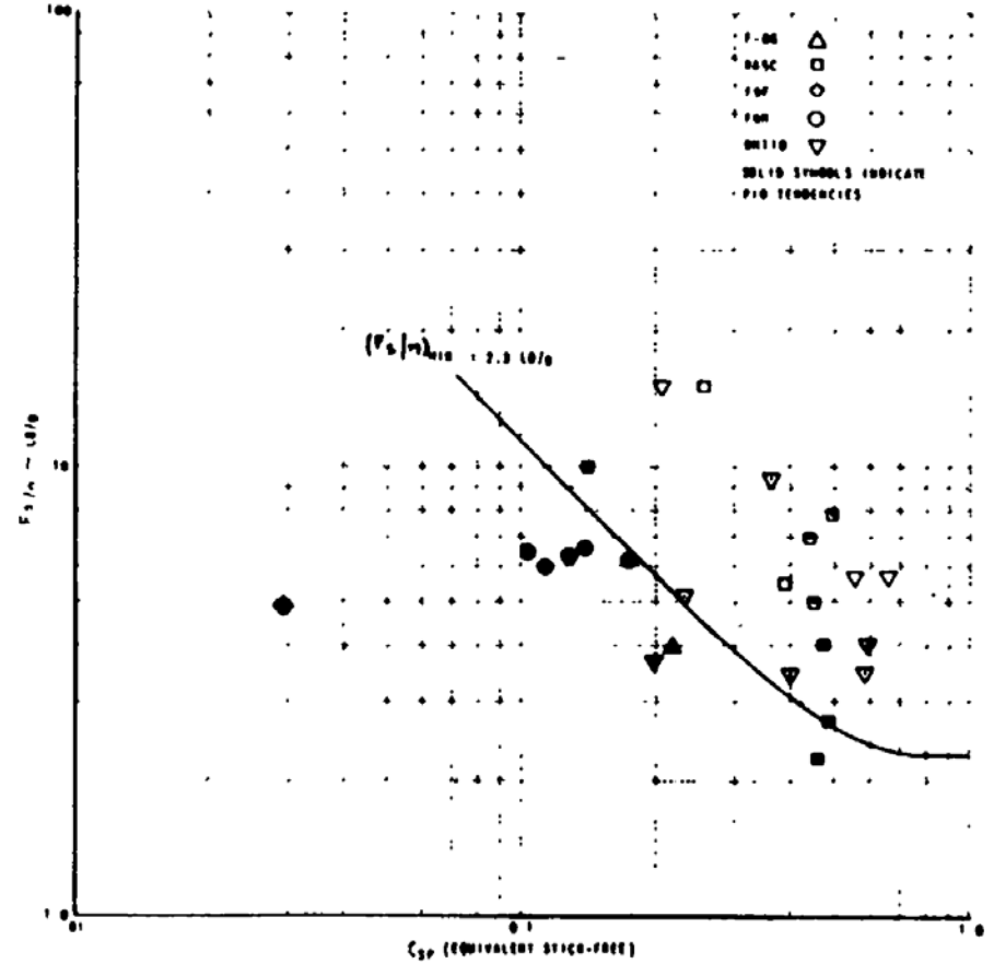
FIGURE 120. PIO characteristics of airplanes described in AGARD-CP-17.
