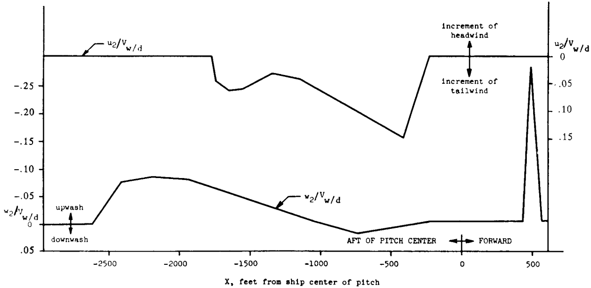
FIGURE 268. CVA ship burble steady wind ratios.
