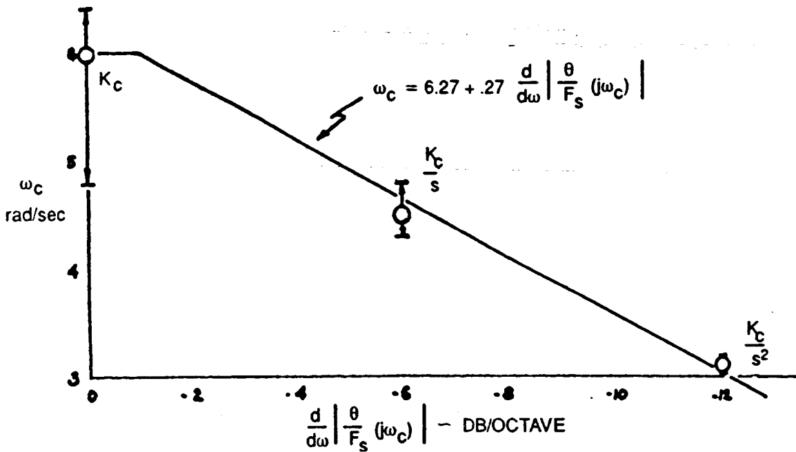
FIGURE 277. Specification of the Criterion Frequency.
