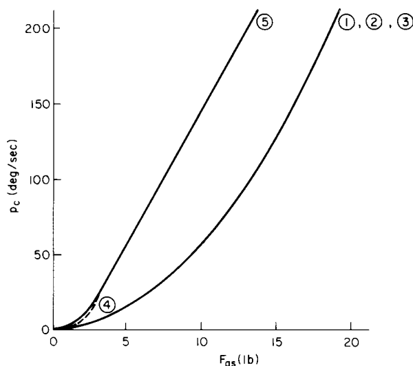
FIGURE 199. Evolution of roll CAS network for YA-7D DIGITAC (AFFTC-TR-76-15).
