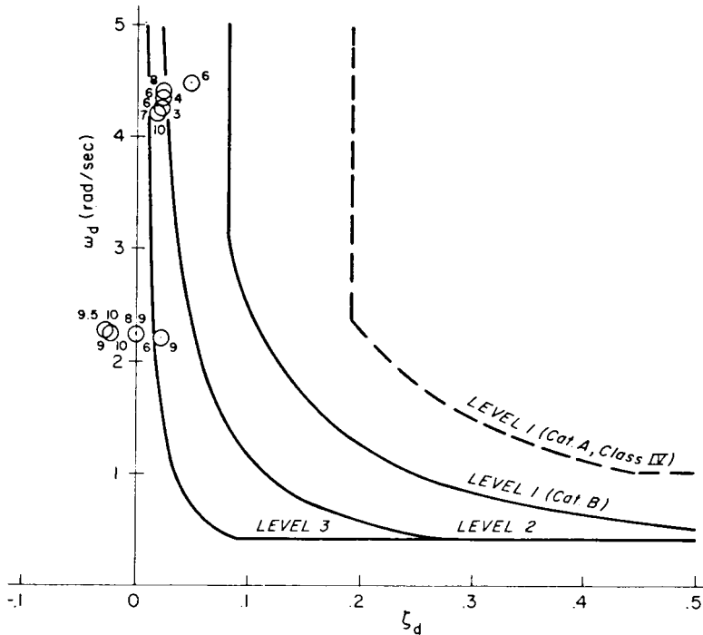
b) 25.0 \leq \omega_d^2 |\phi/\beta|_d \leq 28.8 (rad/sec)^2 ; Boundaries Drawn for 27.0
