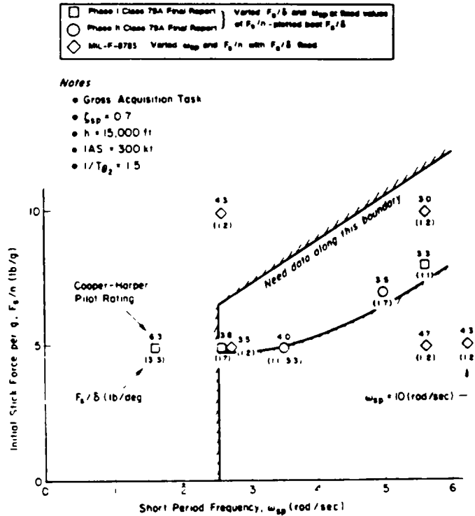
FIGURE 104. Short-period frequency vs longitudinal stick force per g ( F_S/\delta separately optimized) for a side-stick controller.
