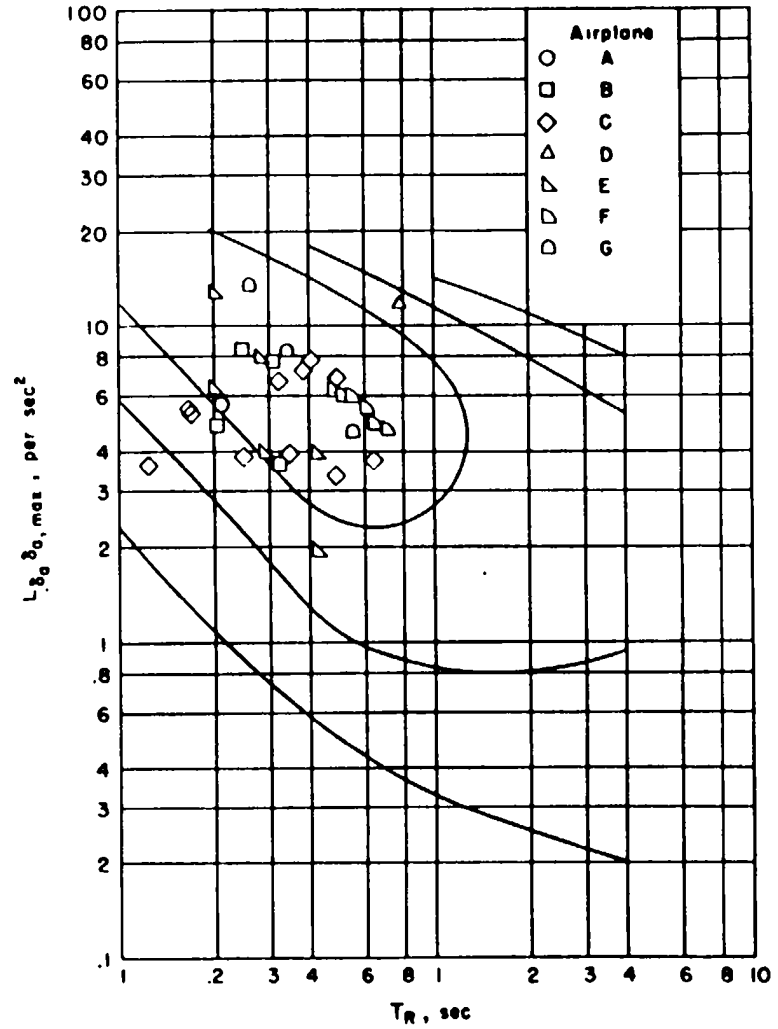
FIGURE 141. Range of parameters L_{\delta_a} \delta_{a_{max}} and T_R covered in the flight investigation, shown in comparison with the motion simulator driven boundaries (from NASA Memo 1-29-59A).
