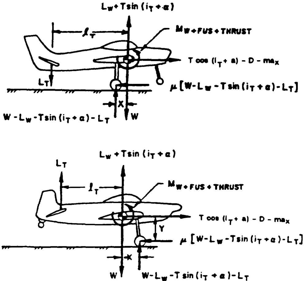
FIGURE 96. Nosewheel and tailwheel lift-off.
