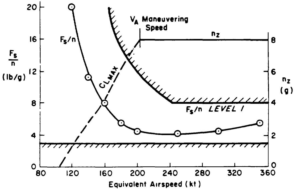
FIGURE 102. OV-10A maneuvering control (AFFDL-TR-78-171).
