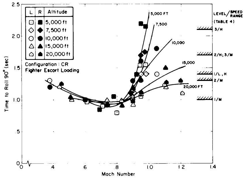
FIGURE 183. Time to roll 90° versus mach for F/A-18A (Navy Rpt No. SA-14R-81).
