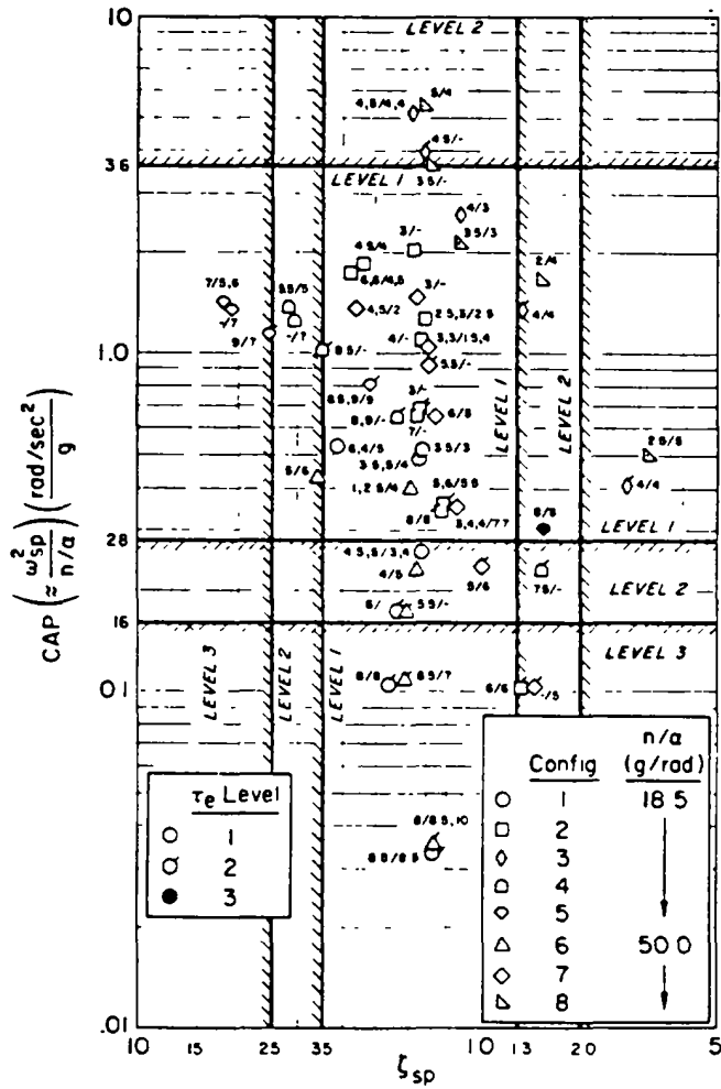
a) \zeta_{sp} and \omega_{sp} Requirements
