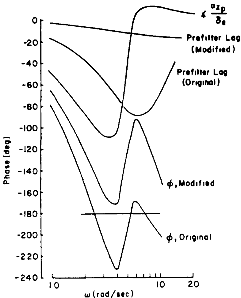
FIGURE 93. YF-17 acceleration control system dynamics (AFFDL-TR-77-57).
