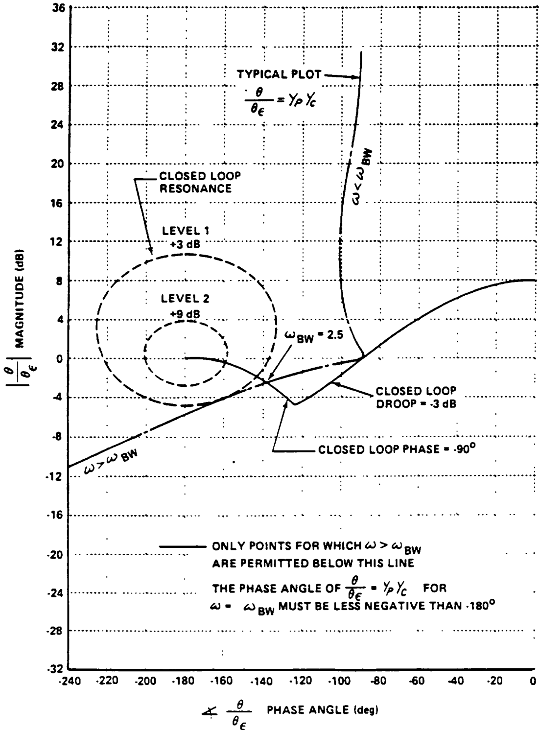
FIGURE 68. Design criteria for pitch dynamics with the pilot in the loop.
