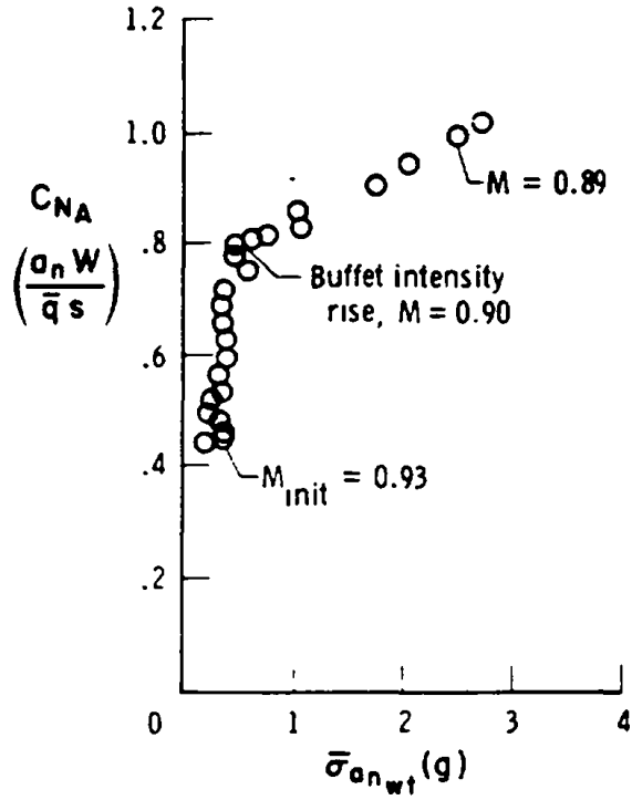
a) Normalized RMS Values of Wingtip Normal Acceleration
