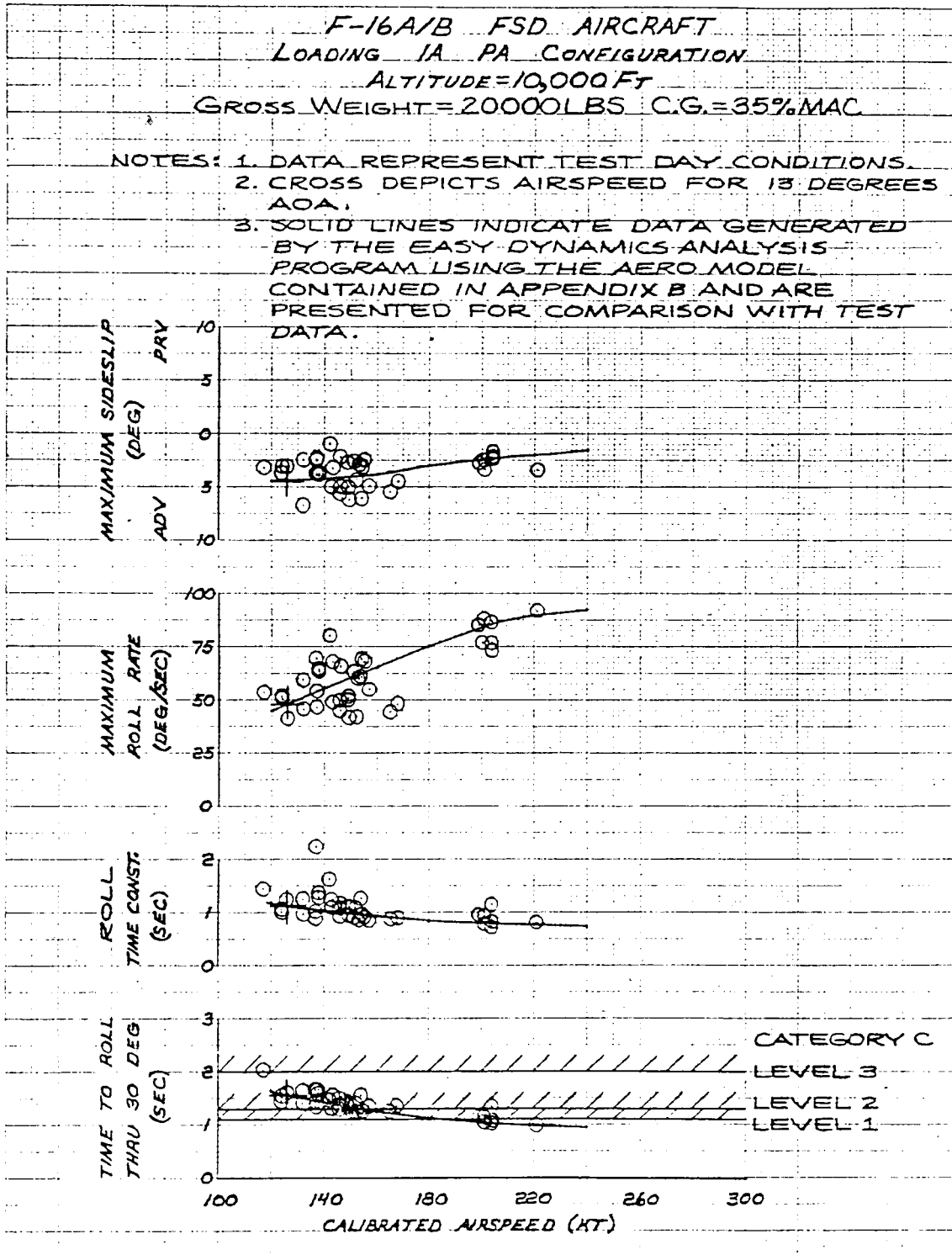
FIGURE. 188. Roll performance summary (from AFFTC-TR-79-10).
