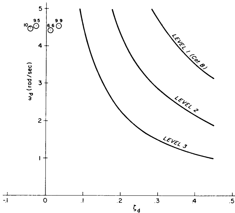
d) 97.9 \leq \omega_d^2 |\phi/\beta|_d \leq 116.5 \text{ (rad/sec)}^2 ; Boundaries Drawn for 110.0
