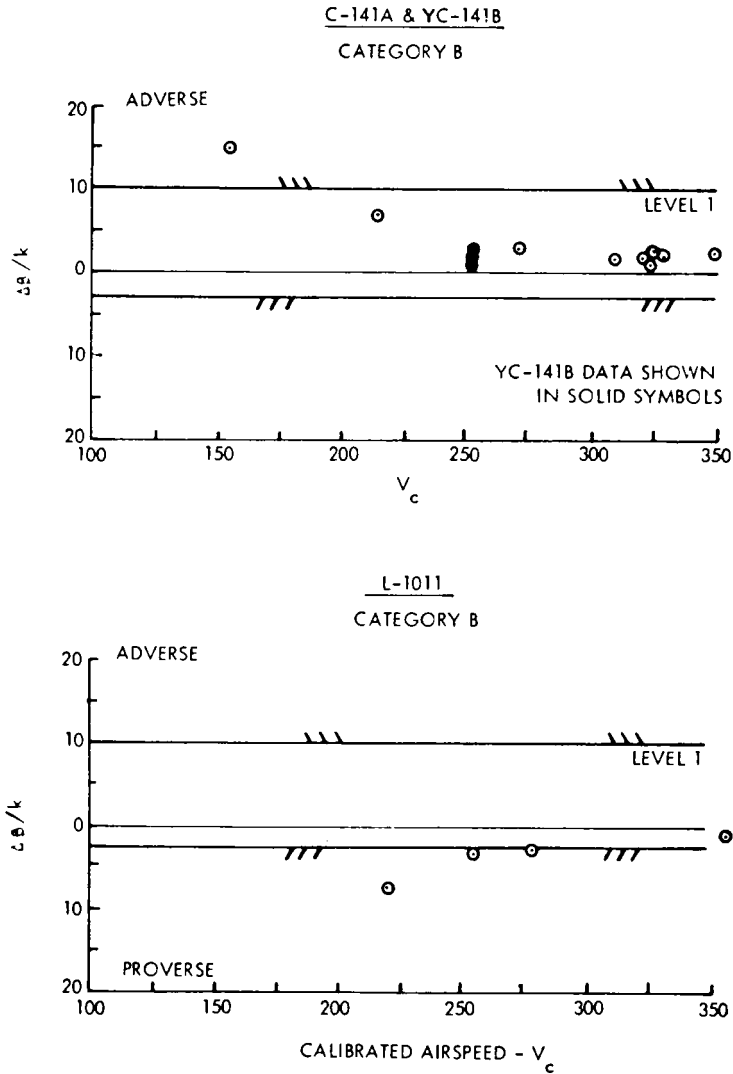
FIGURE 244. Sideslip excursion data for Class III aircraft in Category B Flight Phases (from AFFDL-TR-78-171)
