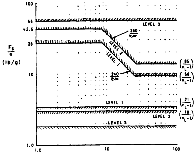
FIGURE 100. Elevator maneuvering force gradient limits: center-stick controller, n_L = 7.0 .
