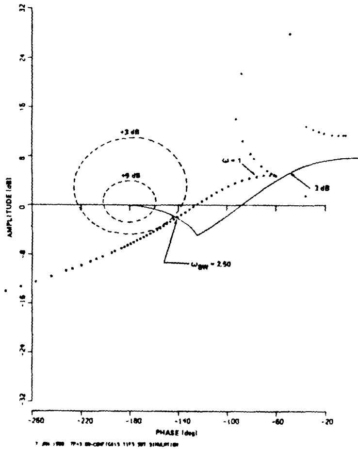
FIGURE 69. Amplitude-phase plot for configuration 13 (fwd; c.g.).
