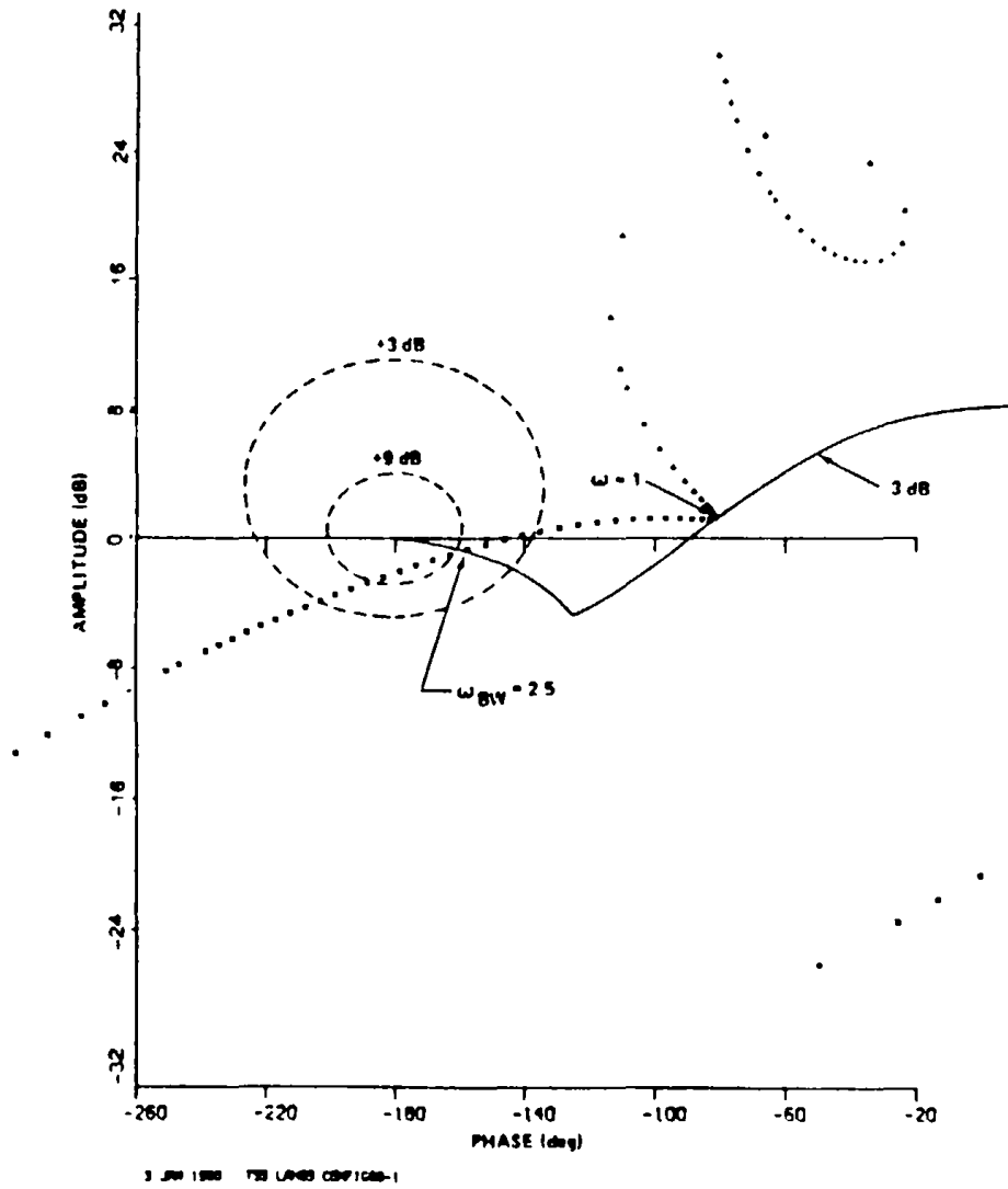
FIGURE 71. Amplitude-phase plot for configuration 6-1.
