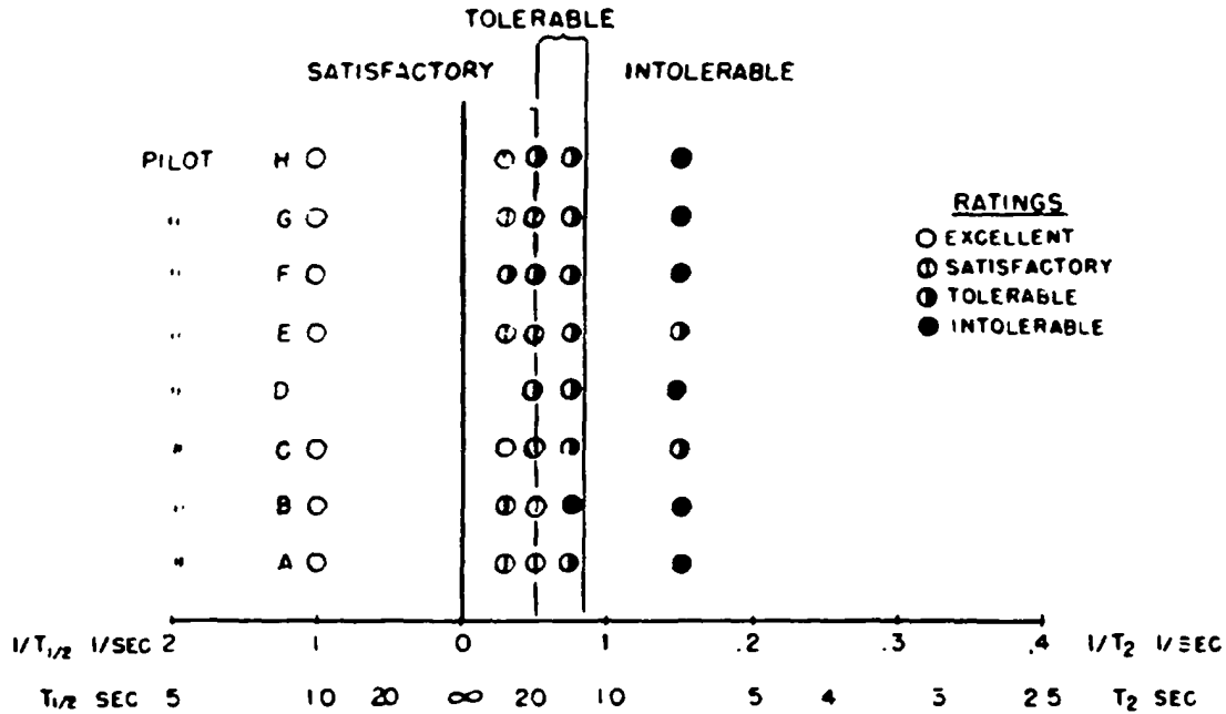
FIGURE 148. Limits of satisfactory and tolerable rates of spiral divergence (from Cornell Aero Lab TB-574-F-6).
