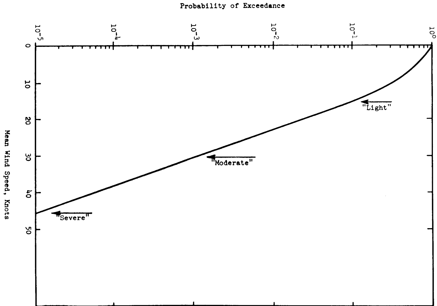
FIGURE 263. Probability of exceeding mean wind speed at 20 ft.
