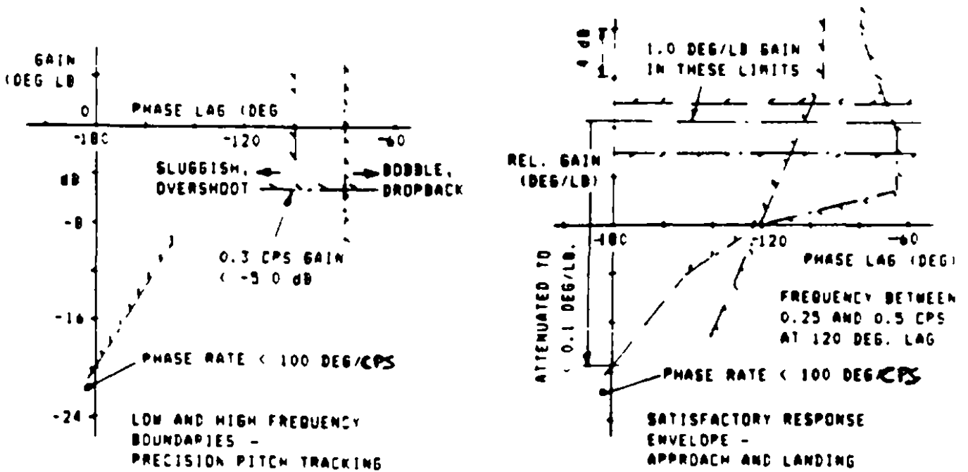
FIGURE 74. Equivalent \omega_n boundaries.
