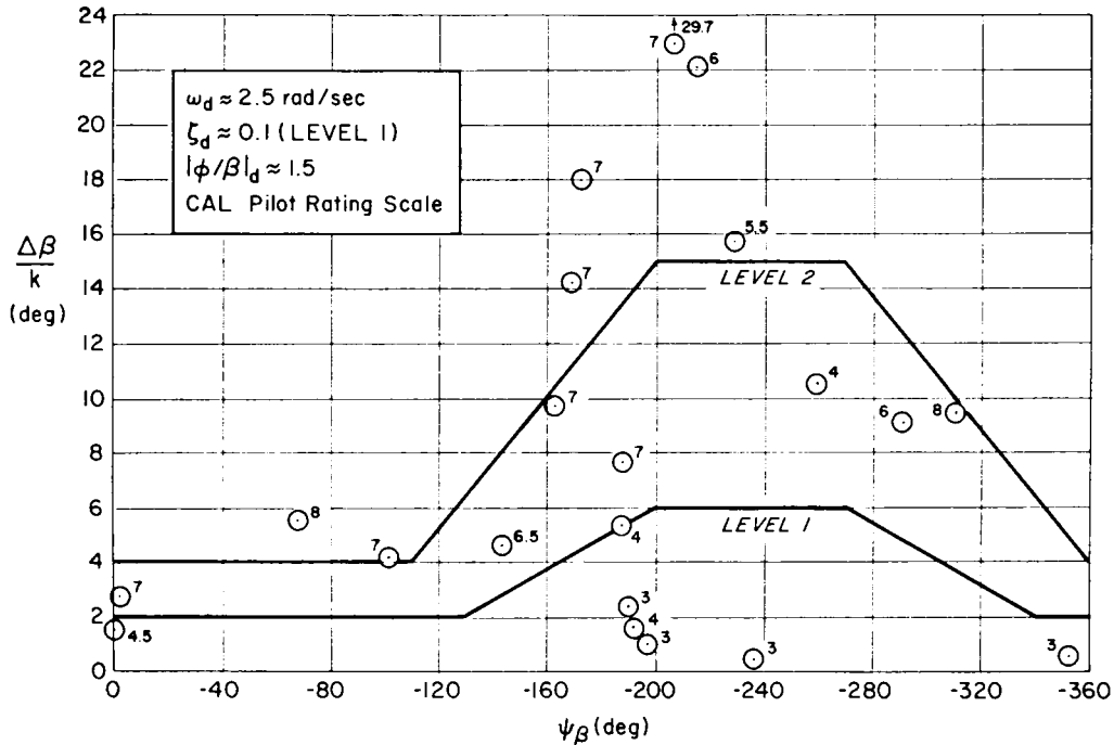
FIGURE 238. Flight Phase Category A data from AFFDL-TR-67-98 (AOIk, from AFFDL-TR-72-41).
