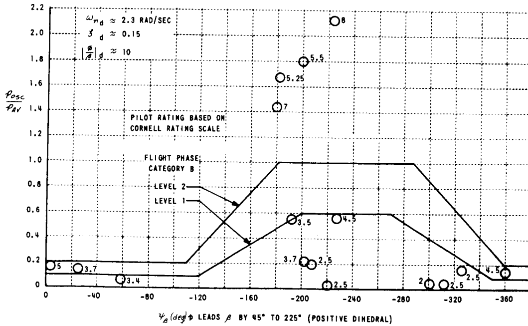
FIGURE 163. Flight phase Category B data (from NASA-CR-778).
