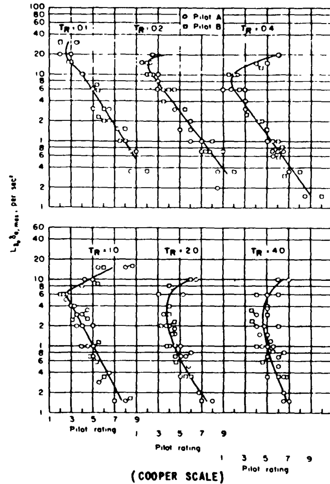
FIGURE 139. Variation of pilot opinion with L_{\delta_a} \delta_{a_{max}} for constant values of T_R as obtained from the moving flight simulator (from NASA Memo 1-29-59A).
