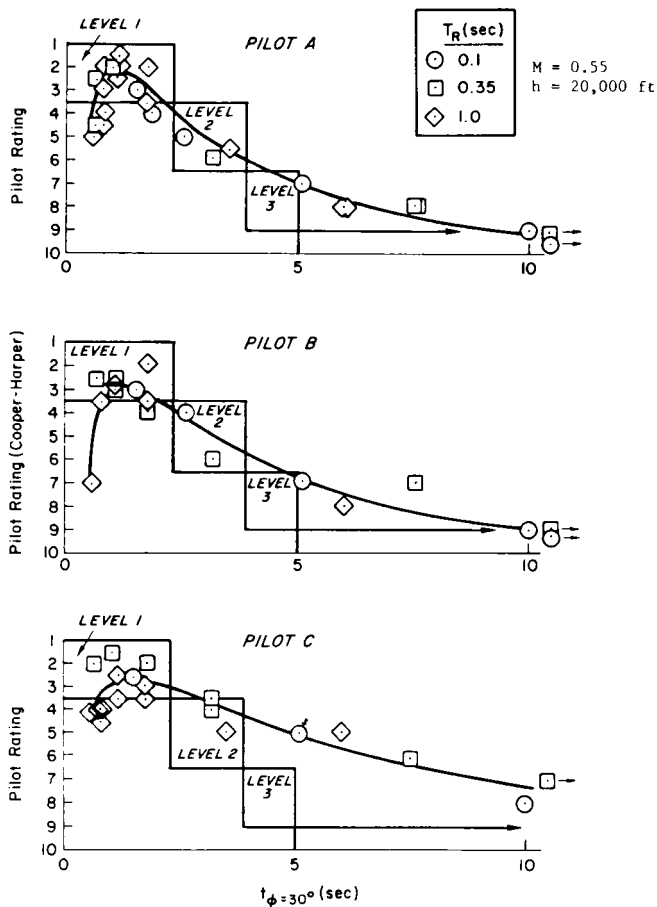
FIGURE 175. Comparison of pilot ratings for Class III aircraft in Category B Flight Phases with requirements of table XXIX (NASA-TN-D-5957).
