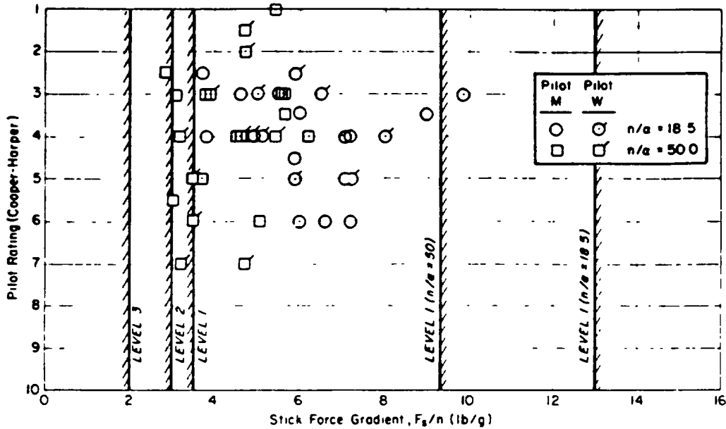
FIGURE 107. Comparison of optimum F_S/n from data of Neal and Smith (AFFDL-TR-70-74) with limits of table XVII (Category A; n_L = 7 g).
