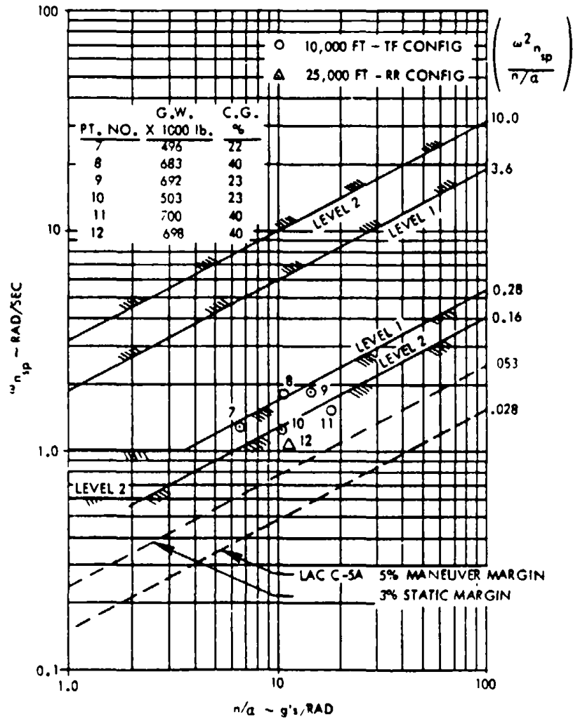
FIGURE 28. Category A C-5A flight test data.
