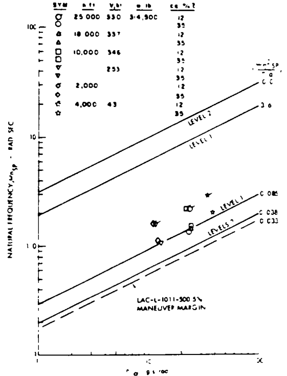
FIGURE 33. L-1011 climb short-period characteristics.
