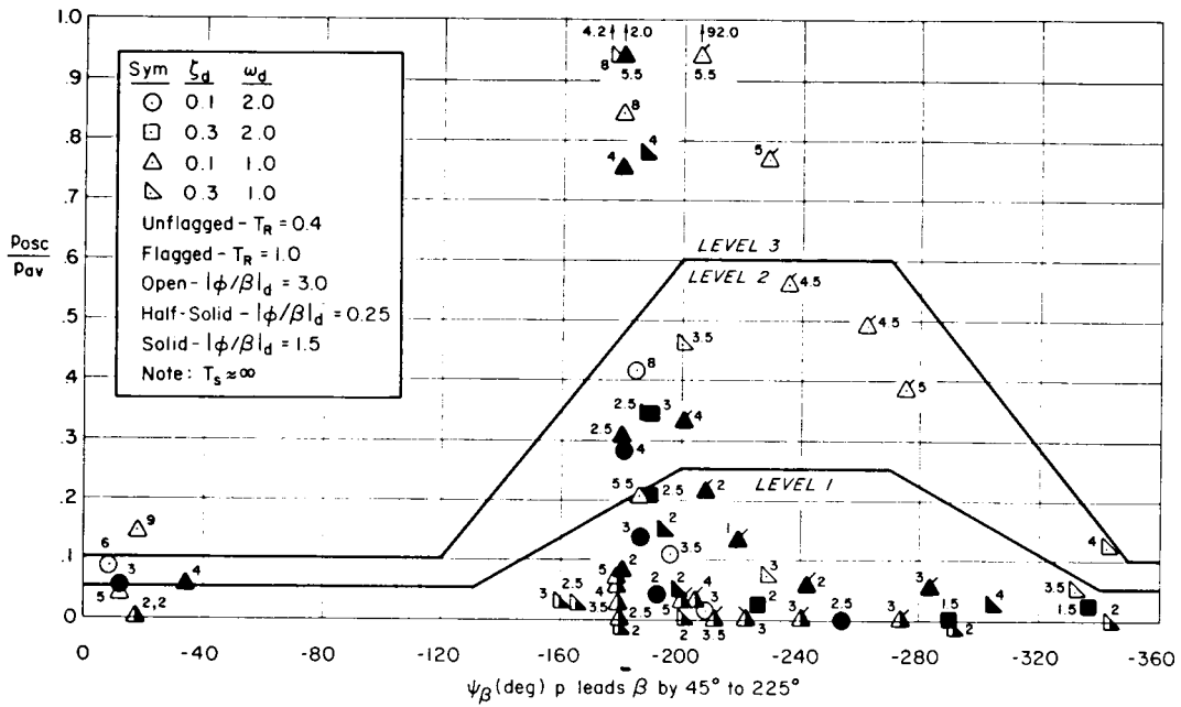
FIGURE 166. Category C data (approach and wave-off); Cooper-Harper pilot ratings (from AFFDL-TR-70-145).
