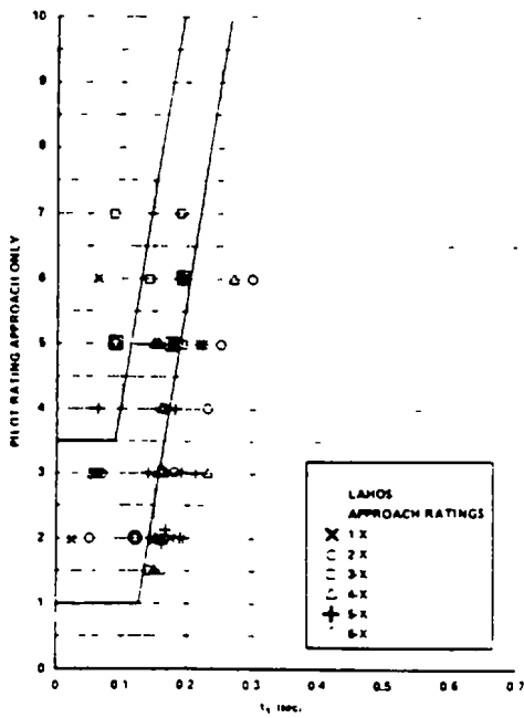
FIGURE 54. Pilot rating correlation with effective time delay (AFFDL-TR-78-122).
