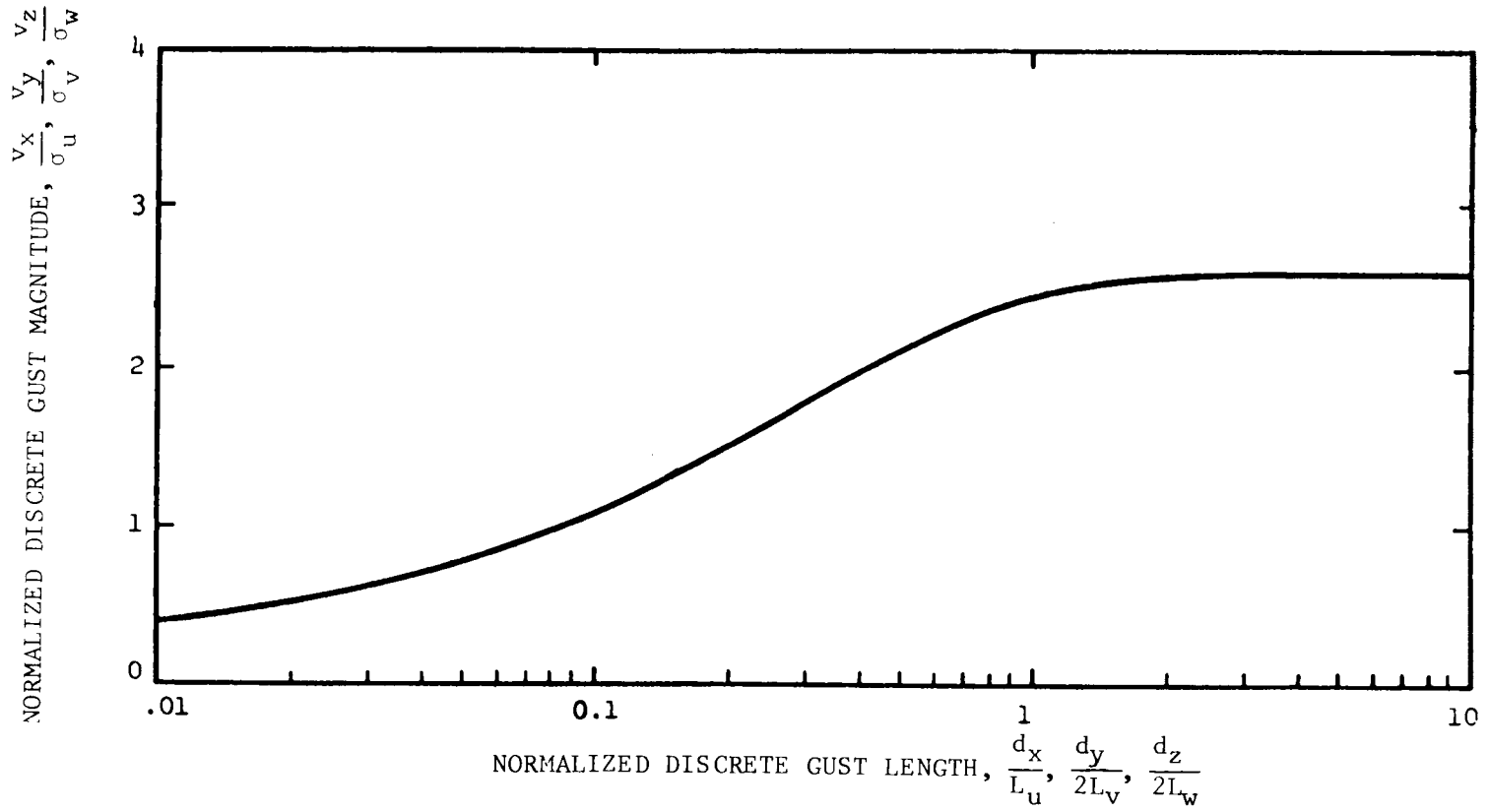
FIGURE 265. Magnitude of discrete gusts.
