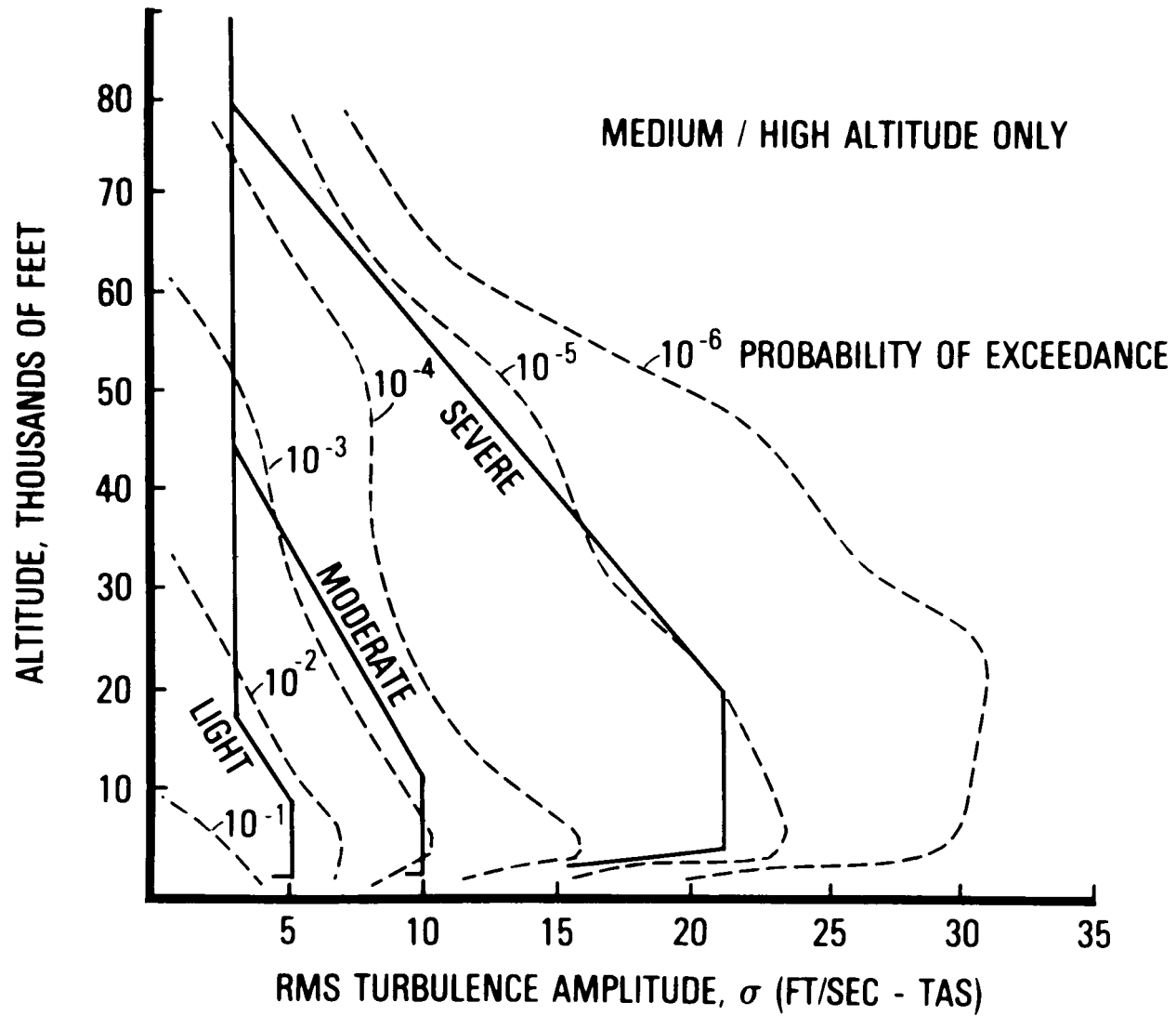
FIGURE 262. Turbulence severity and exceedance probability.
