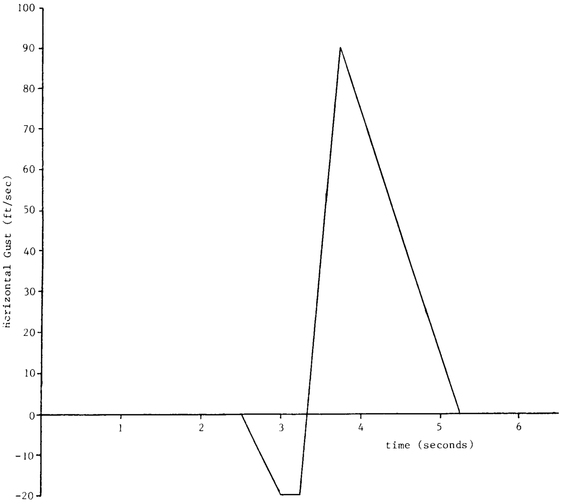
FIGURE 264. Earth-axis winds.
