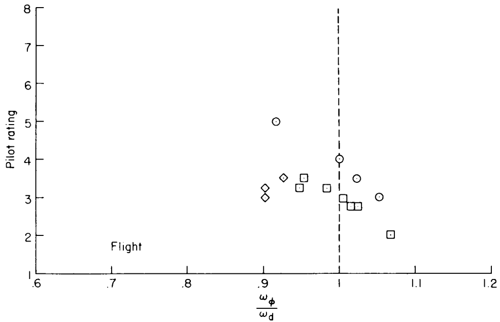
FIGURE 222. Variation of pilot rating with \omega_\psi/\omega_d for moving-base simulator and flight data \zeta_d \approx 0.15 (NASA-TN-D-3910).
