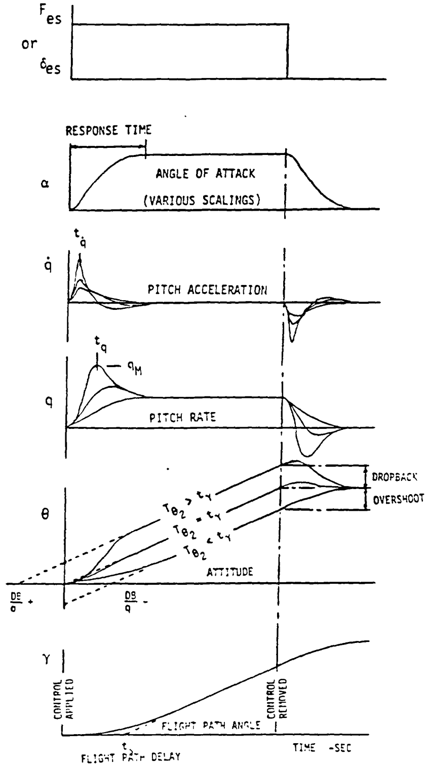
FIGURE 73. Pitch short period time responses.
