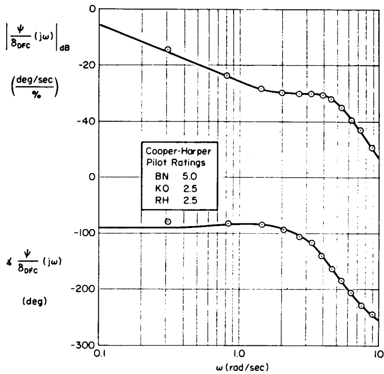
FIGURE 89a. Typical DFC control frequency sweep.
