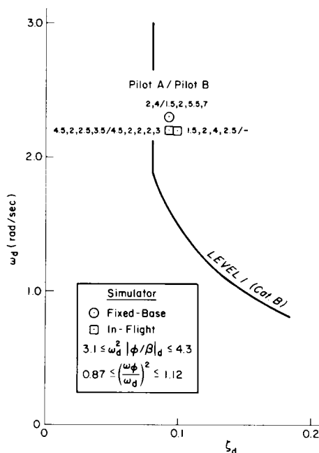
FIGURE 212. Dutch roll data (from NASA-CR-778; low \omega_d^2 |\phi/\beta|_d ).
