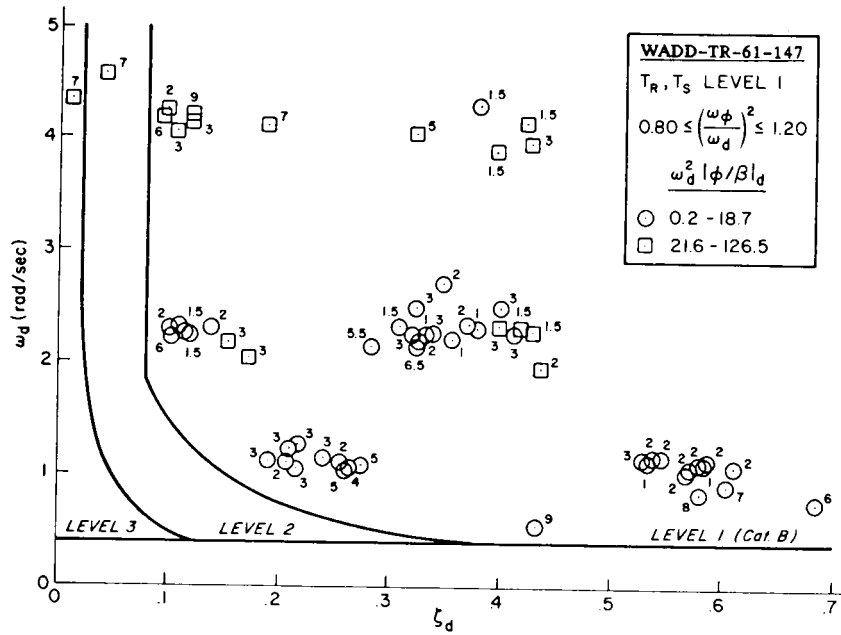
FIGURE 214. Dutch roll data (from WADD-TR-61-147).
