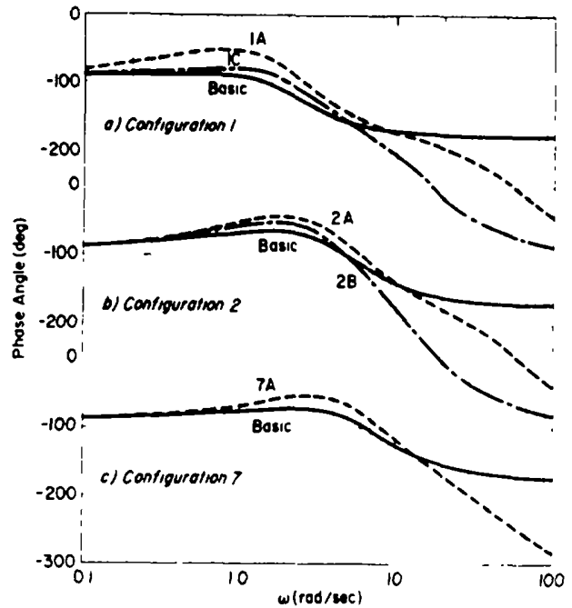
FIGURE 17. Comparison of phase angles for basic and augmented configurations of table XIII.
