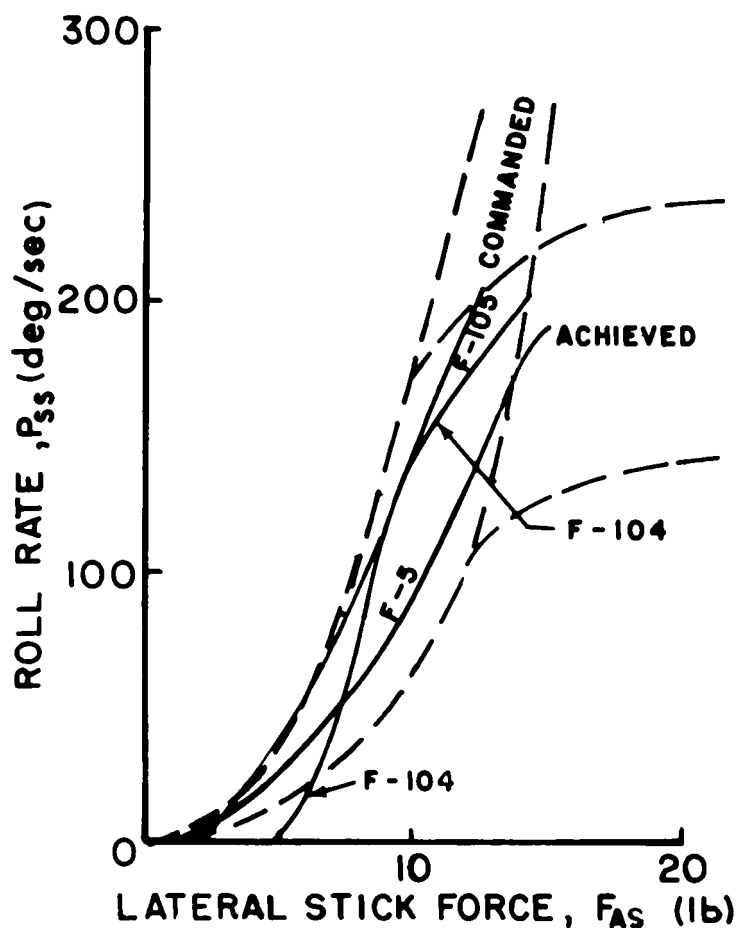
FIGURE 195. Comparison Of P_{max} @ F_{as} for several conventional Class IV aircraft with CAS curves of figure 194.
