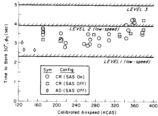
a) Category B Flight Phases
