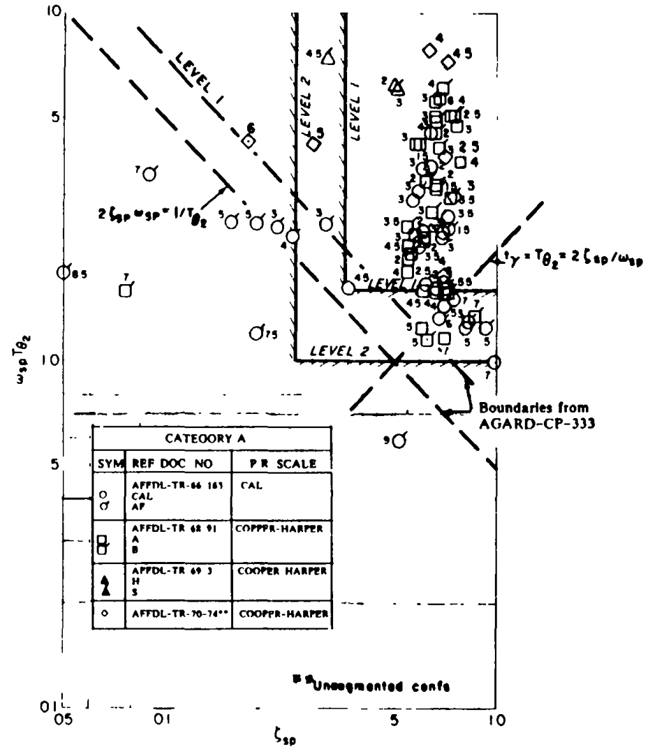
FIGURE 29. Alternate Category A flying qualities requirements for short-period pitch response.
