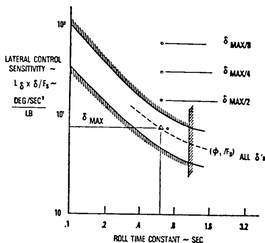
FIGURE 204. Typical roll sensitivity - high gain.
