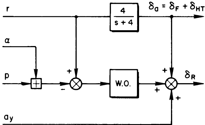
FIGURE 256. Anti-spin SAS for F-16B ( \alpha \geq 29 deg).
