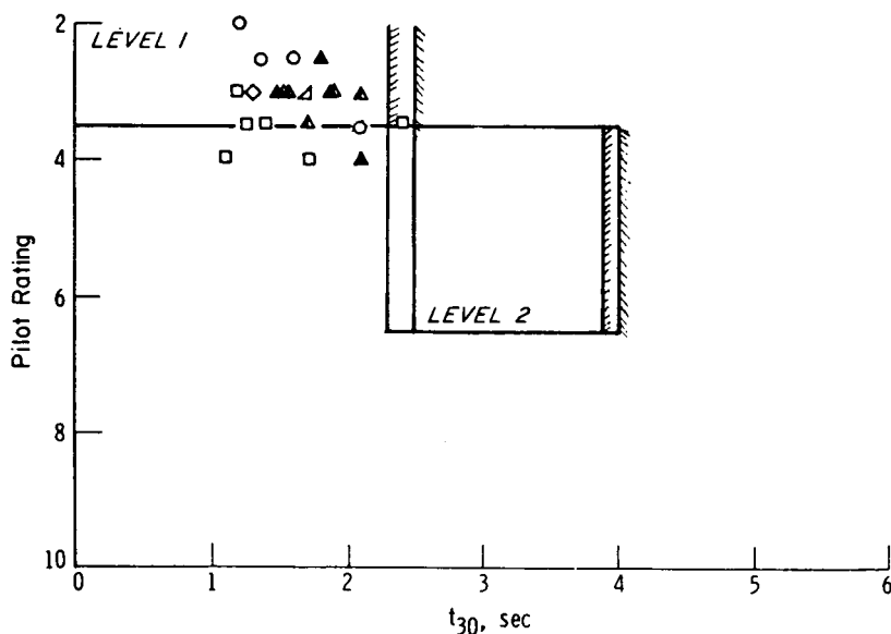
FIGURE 176. Time to bank, 300 for CV-990 (NASA-TN-D-681 1).
