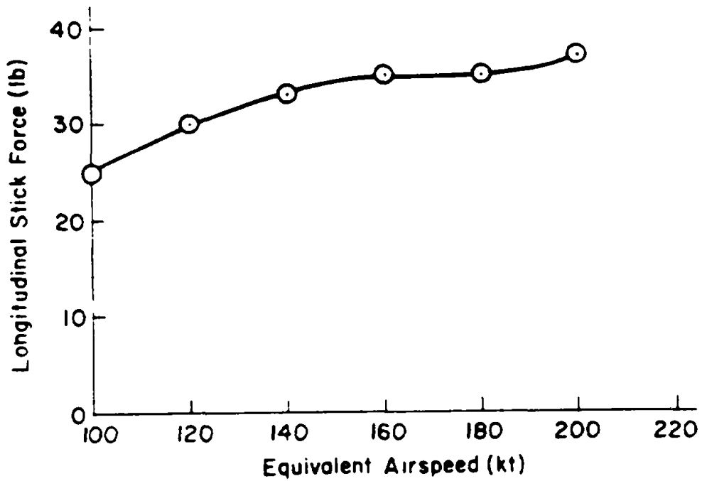
FIGURE 103. Longitudinal stick force at stall (AFFDL-TR-78-171).
