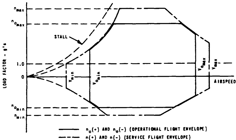
FIGURE 7. Definition of Flight Envelope terms.
