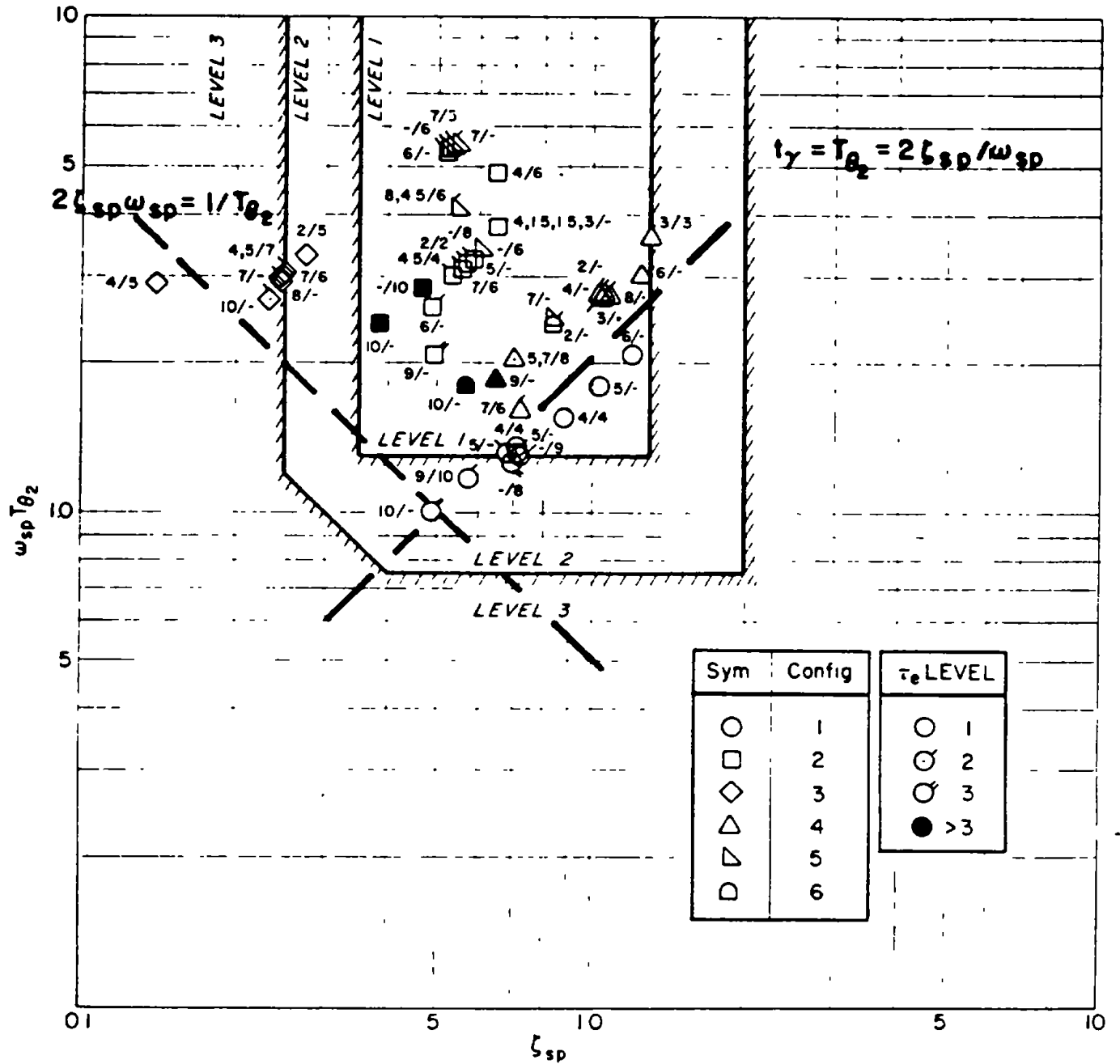
FIGURE 46. Comparison of LAHOS LOES characteristics with \omega_{sp} T_{\theta_2} vs. \zeta_{sp} .
