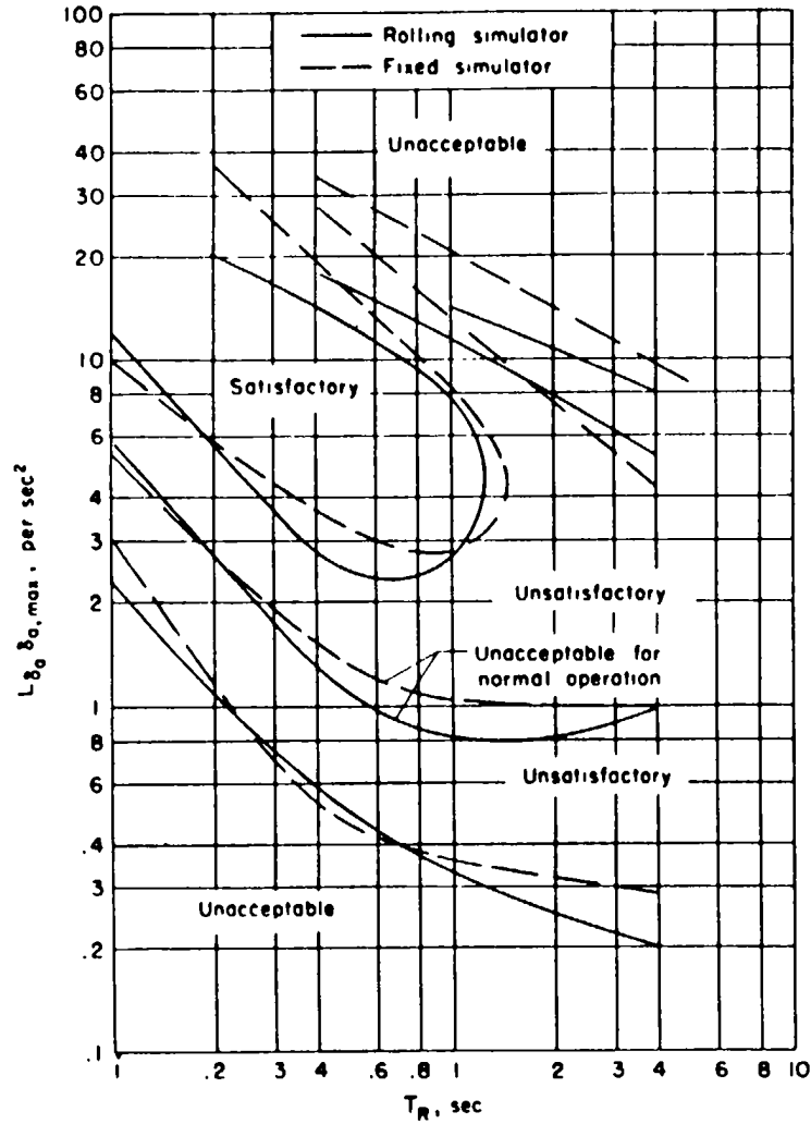
FIGURE 140. Comparison of pilot opinion boundaries obtained from the fixed and moving flight simulators (from NASA Memo 1-29-59A)
