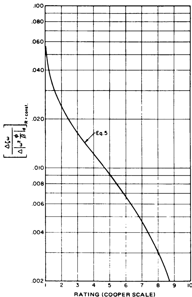
FIGURE 223. \Delta \zeta \omega / \Delta (\omega_d^2 |\phi/\beta|_d) required to maintain a given basic rating (from AFFDL-TR-70-145), based upon data of figures 224 and 225.
