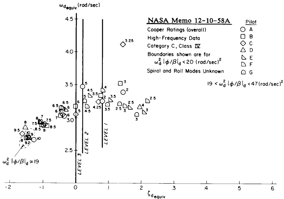
FIGURE 218. Dutch roll data from flight tests of NASA Memo 12-10-58A (F-86E; high-frequency data).
