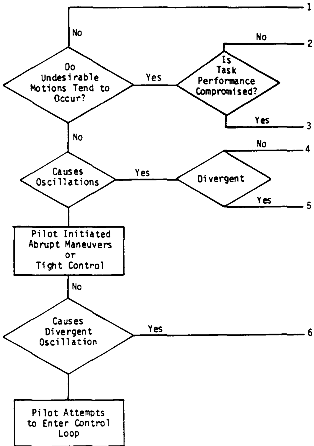
FIGURE 12. PIO tendency classification from AFWAL-TR-81-3118.
