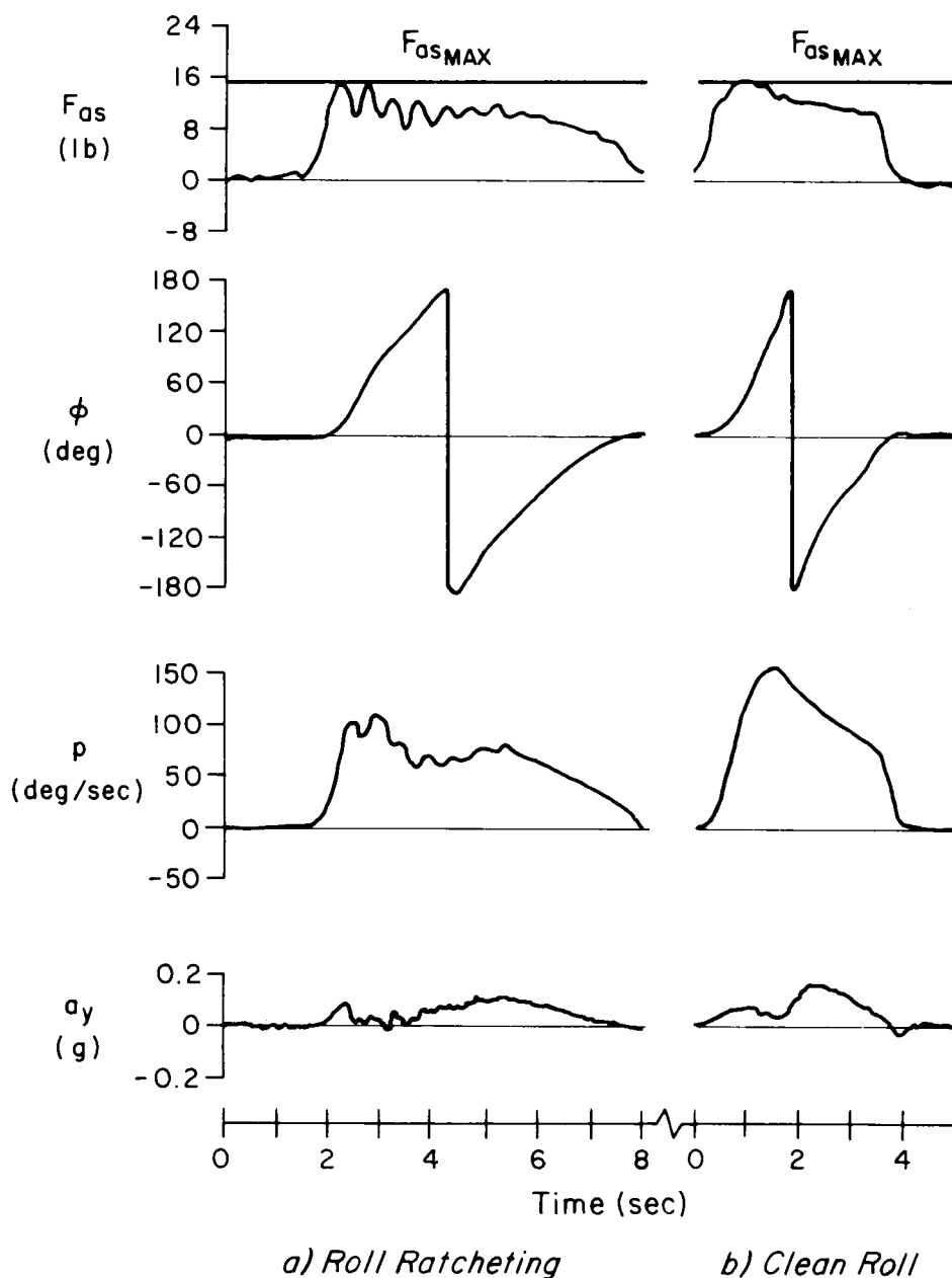
FIGURE 200. Steady rolls on YF-16 (AFFTC-TR-75-15). The roll in (b) was performed 32 seconds after (a) and was satisfactory. h = 10,000 ft, M = 0.80 .
