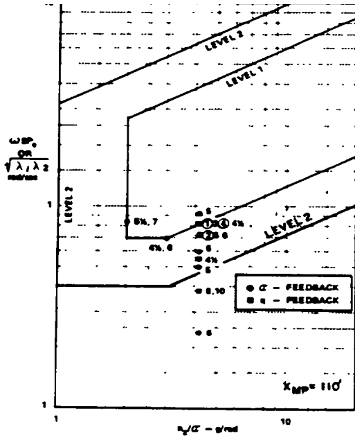
a) Long aft tail, x_{mp} = 110 ft
