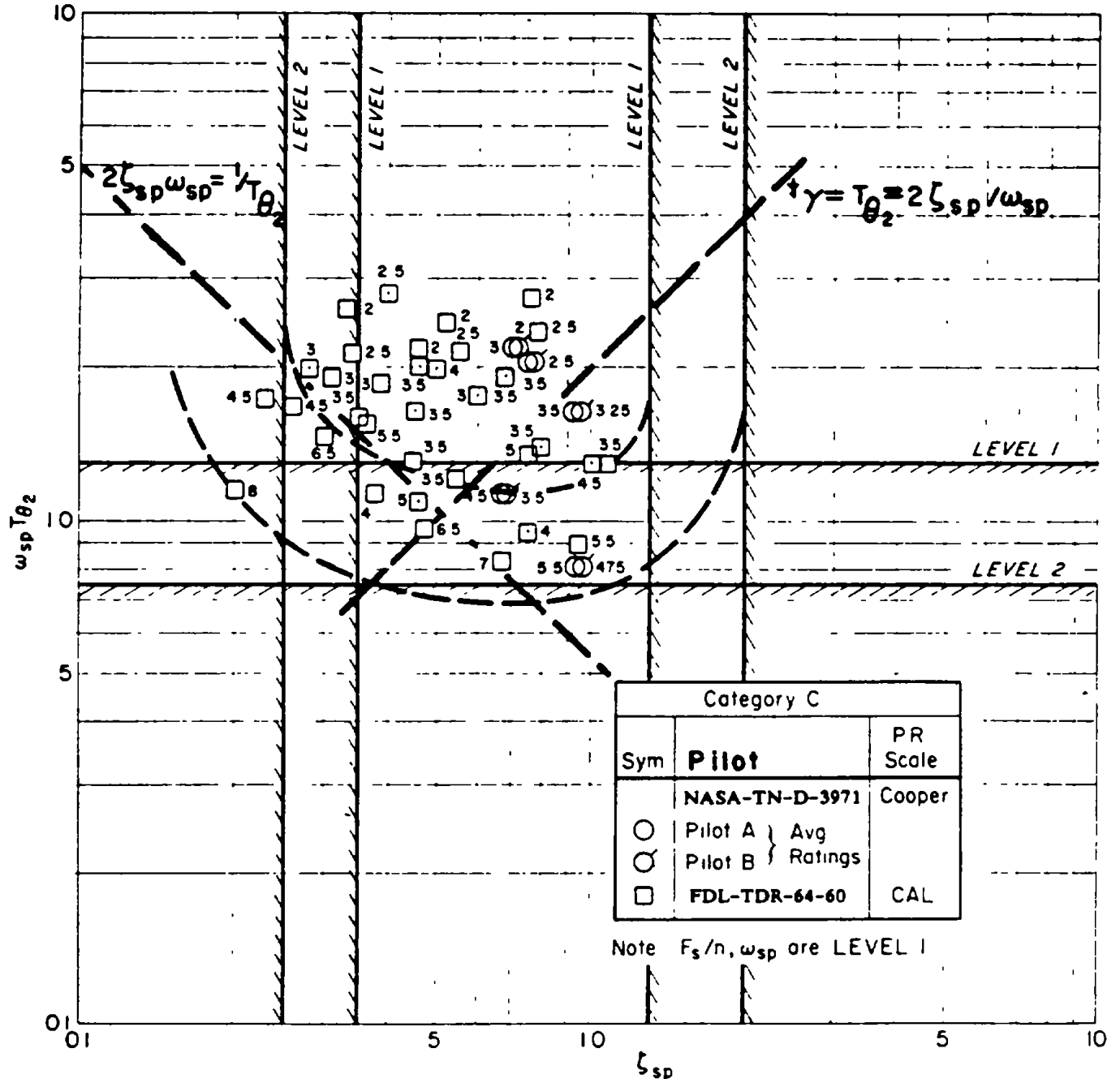
FIGURE 42. Alternate Category C short-period flying qualities requirements.
