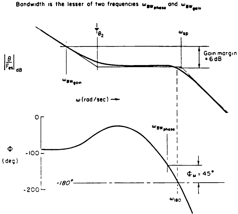
FIGURE 59. Definition of bandwidth frequency \omega_{BW} from open loop frequency response.
