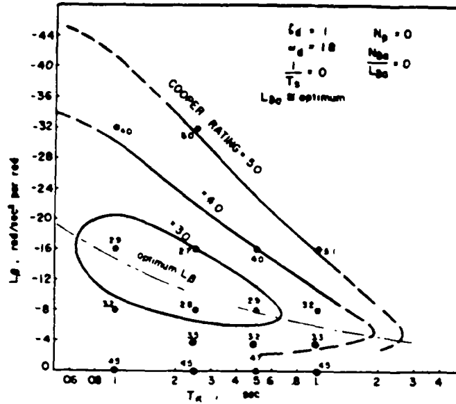
FIGURE 135. Lateral flying qualities boundaries ( L_{\beta} vs. T_R , \zeta_d = 0.1 ) (from Princeton Univ Rpt 727).
