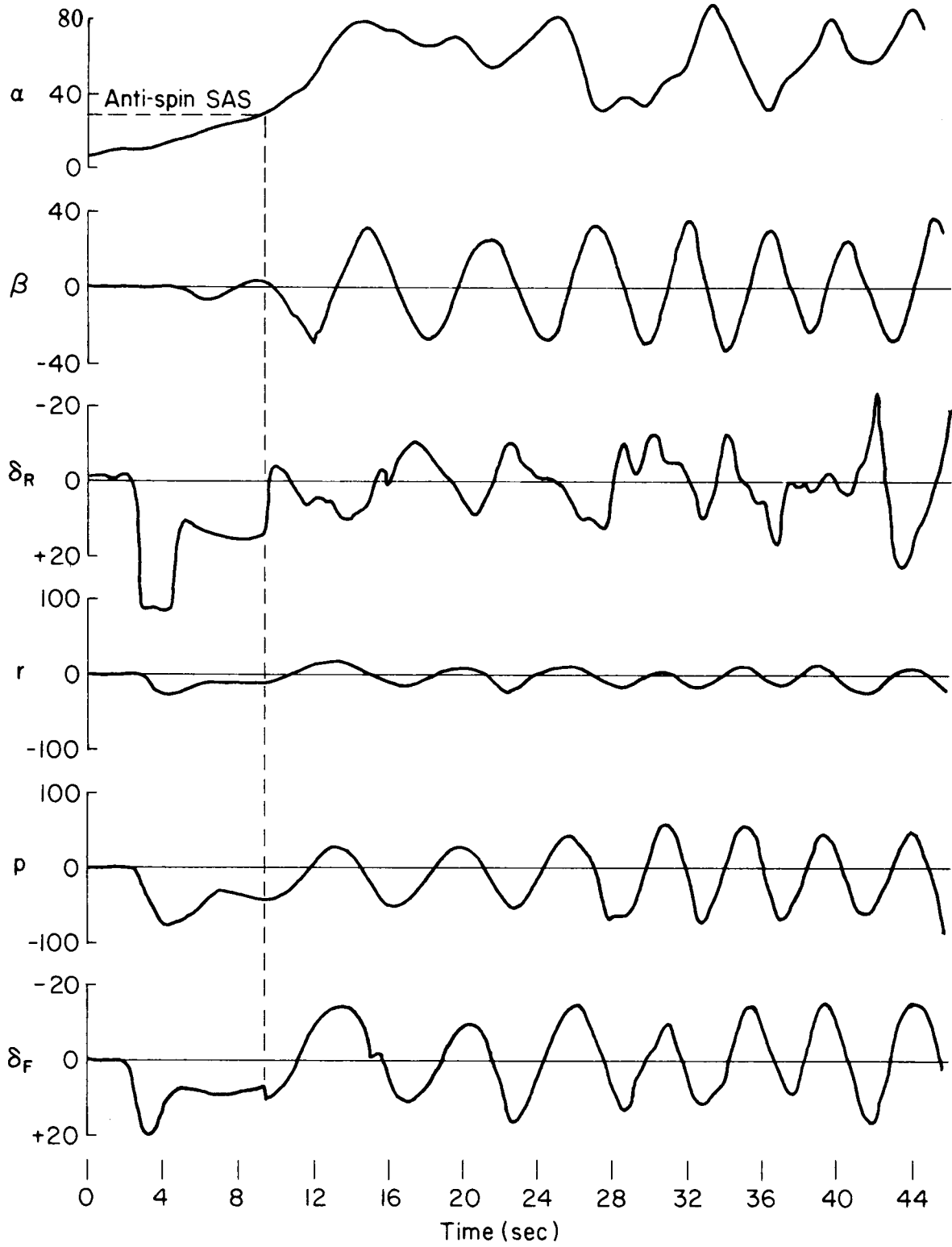
FIGURE 255. Time history of aft-c.g. deep stall encountered by F-16B
