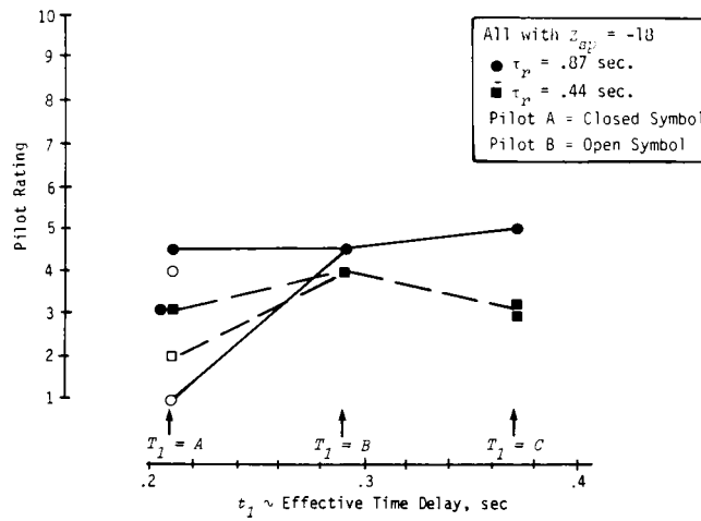
FIGURE 169. Pilot rating vs. time delay -- lateral-directional.
