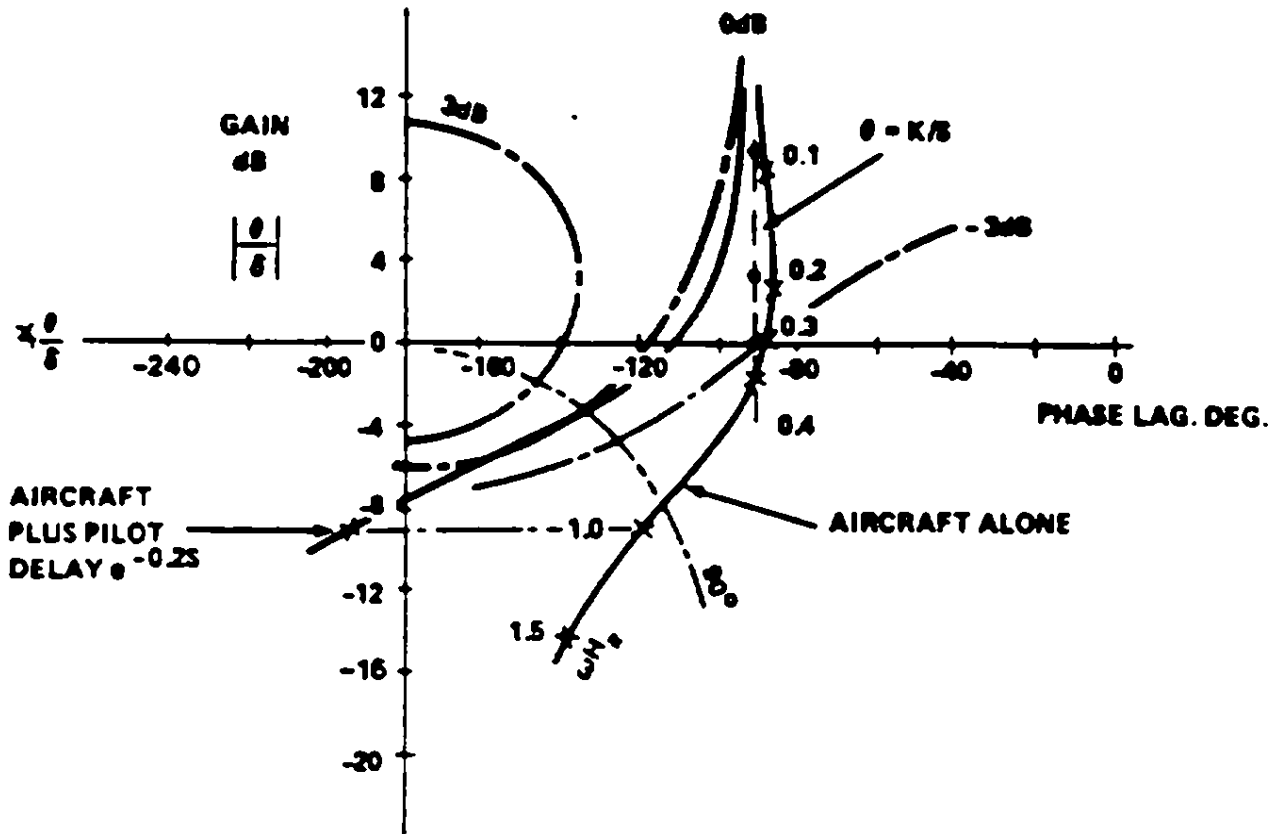
FIGURE 82. Low-order pilot - aircraft attitude frequency response.
