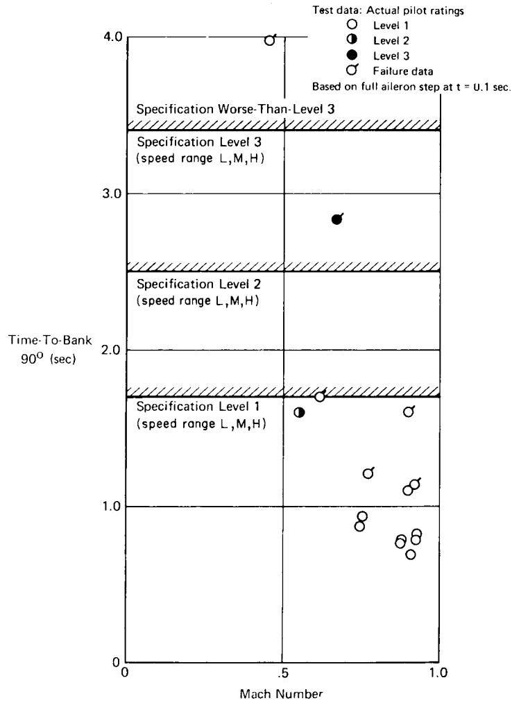
FIGURE 177. F-4 roll control effectiveness, time-to-bank 90^\circ , CR configuration (from AFFFDL-TR-70-155).
