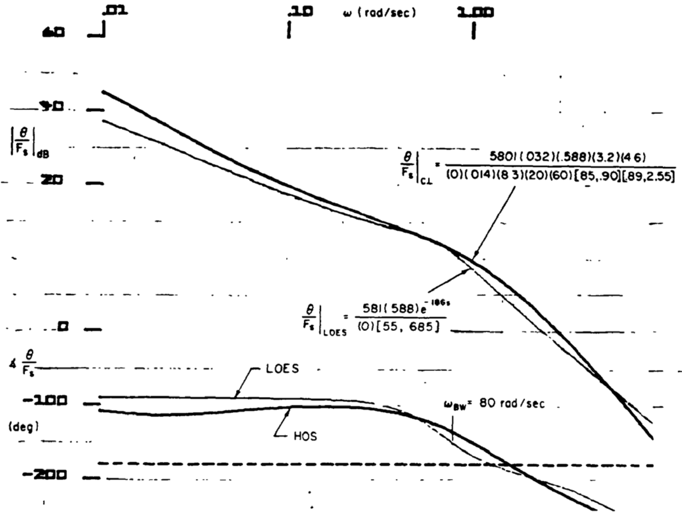
FIGURE 86. AFTI/F-16 \theta \rightarrow F_s for IBU ( q \rightarrow \delta_e closed).
