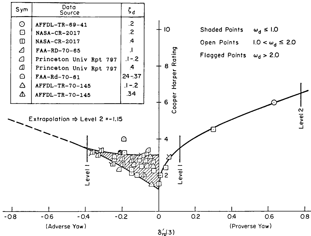
FIGURE 252. Pilot rating correlations when \dot{r}_o/\dot{p}_o is small.
