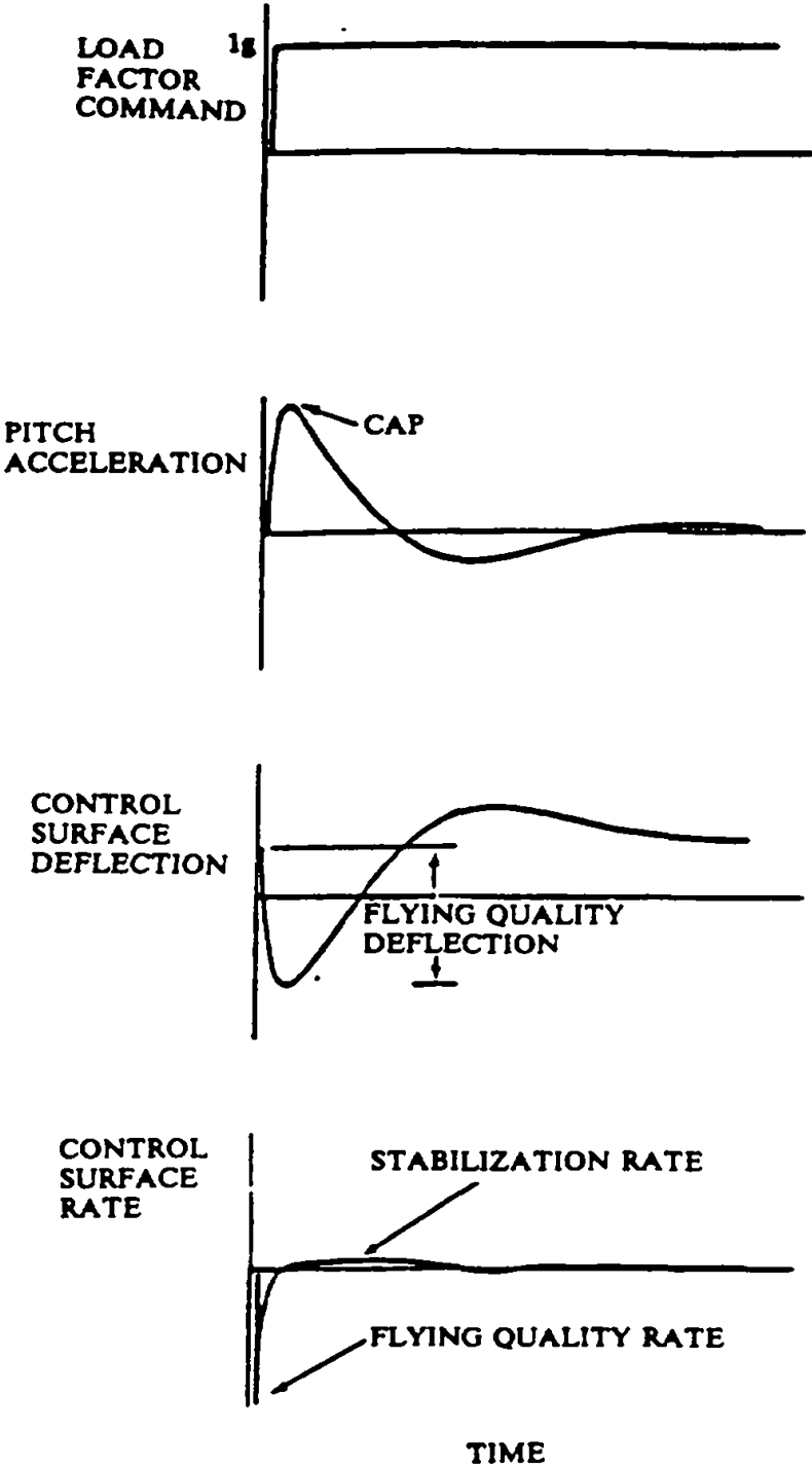
FIGURE 10. Control surface requirements.
