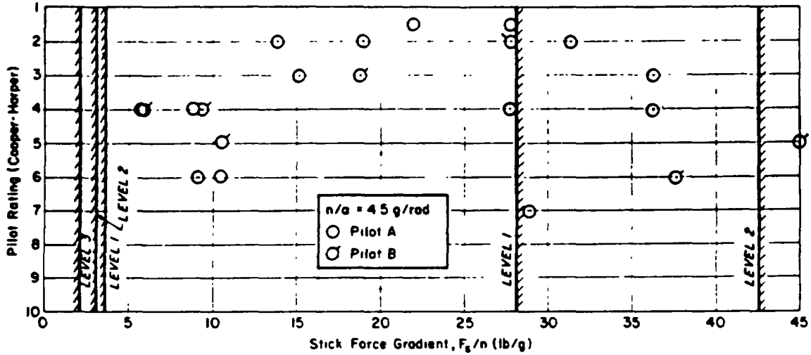
FIGURE 108. Comparison of optimum F_s/n from LAHOS (AFFDL-TR-78-122) data with limits of table XIV (Category C; n_L = 7 g).
