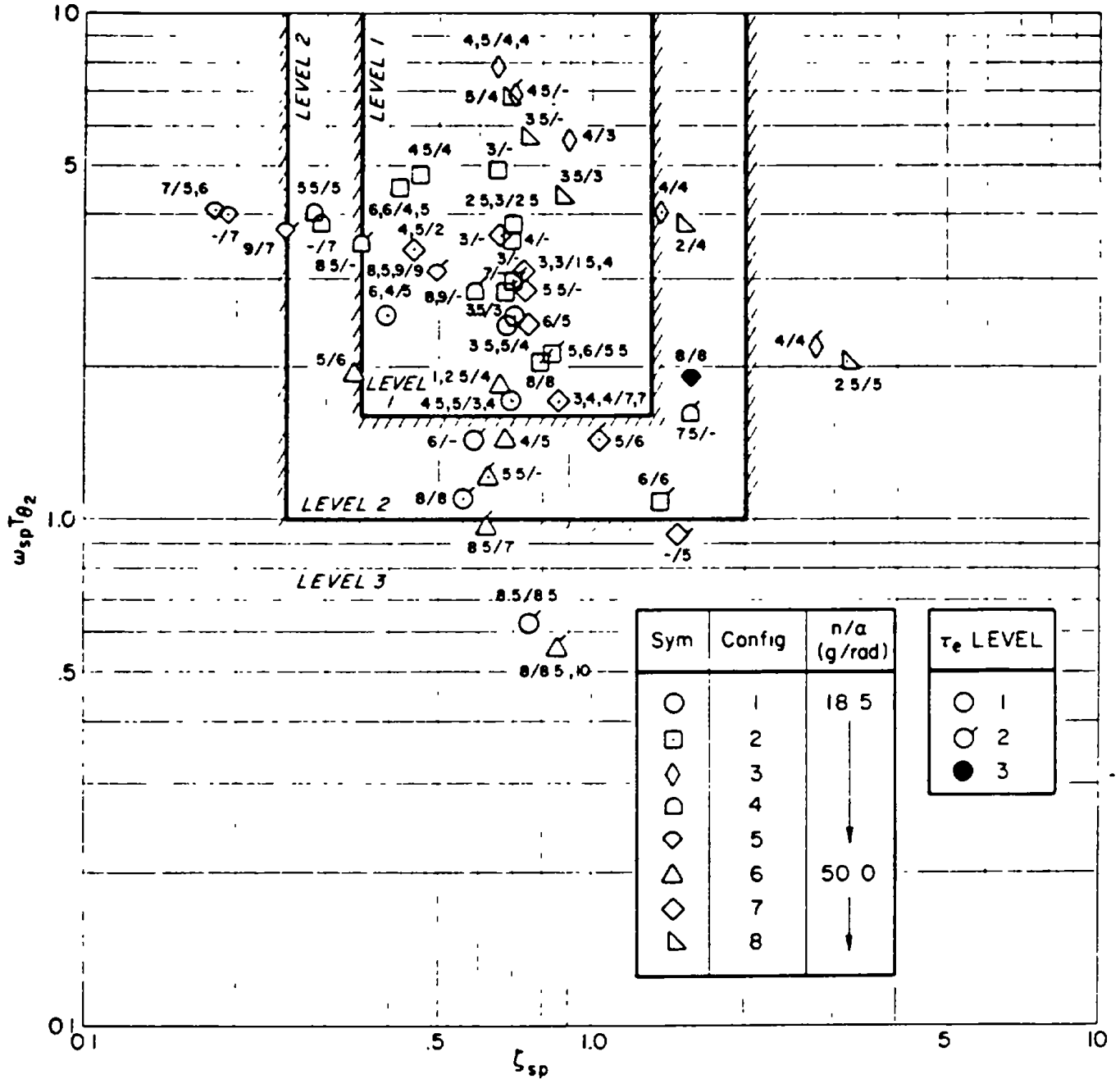
FIGURE 44. Comparison of Neal-Smith LOES characteristics with \omega_{sp} T_{\theta_2} vs \zeta_{sp}
