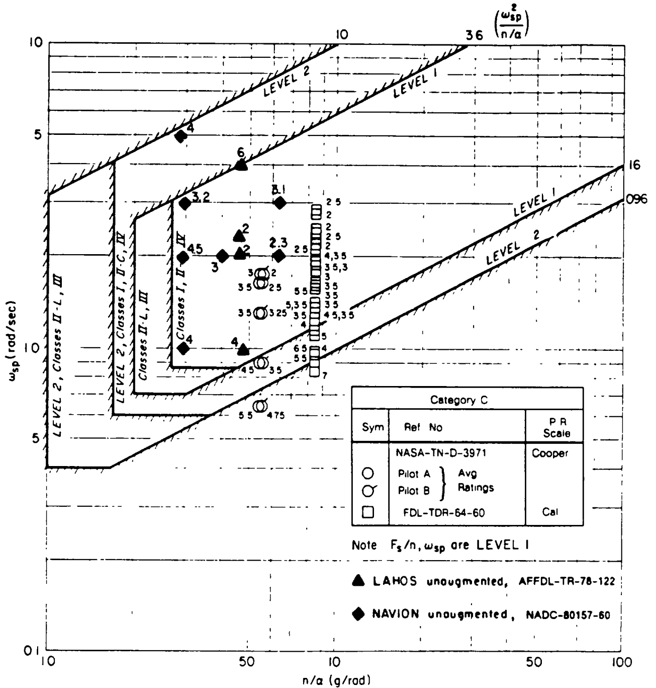
FIGURE 37. Comparison of pilot ratings with Category C short-period frequency requirements.
