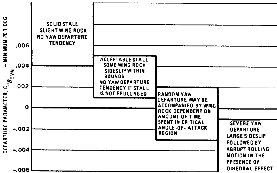
FIGURE 258. Dynamic stability design guide suggested by Titiriga (AGARD-CP-199).
