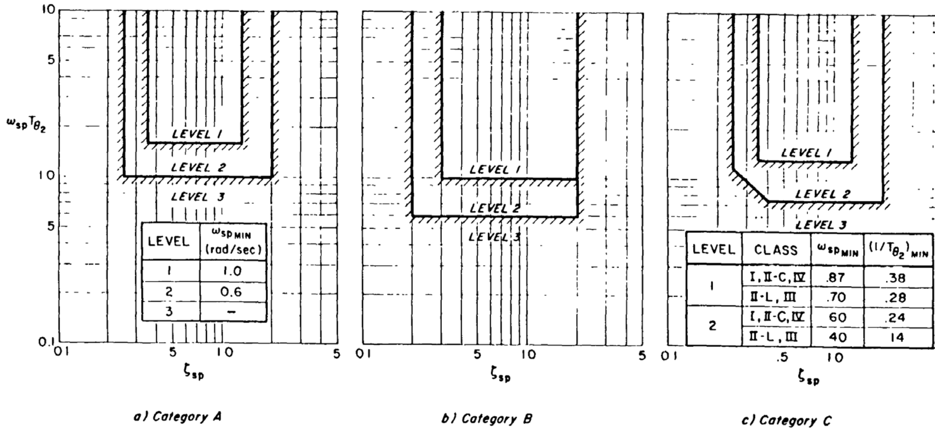
FIGURE 24. Requirements for short-term pitch response to pitch controller ( \omega_{sp}T_{\theta_2} vs \zeta_{sp} ).
