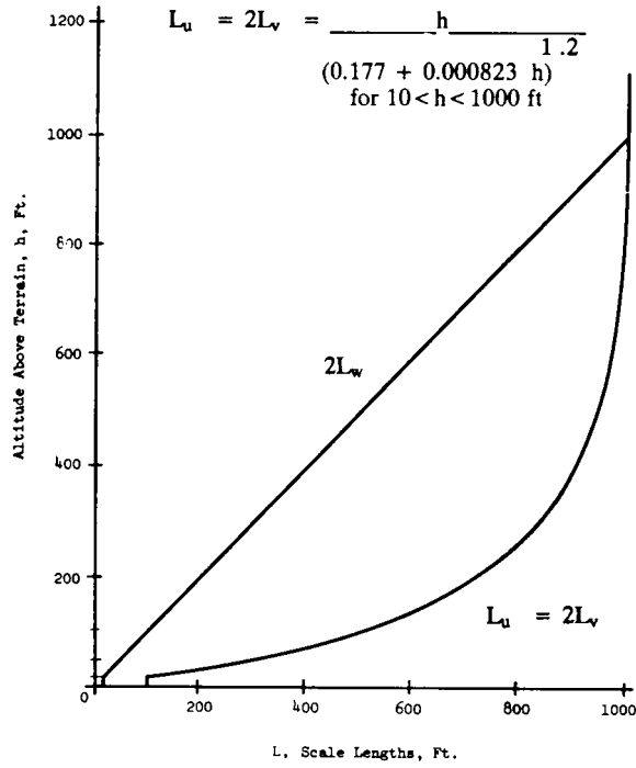
FIGURE 266. Low-altitude turbulence integral scales.
