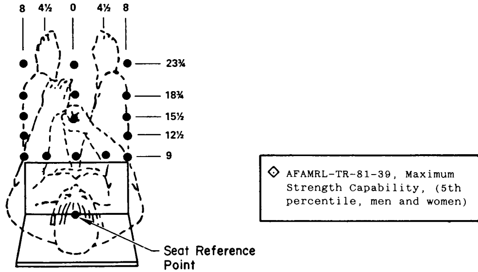
a) Physical Layout For Stick Tests (stick 13 1/2 inches above seat Reference point)
