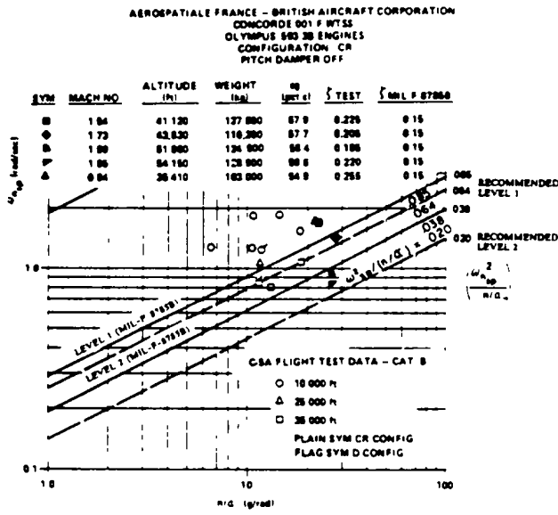
FIGURE 32. Category B short-period characteristics.
