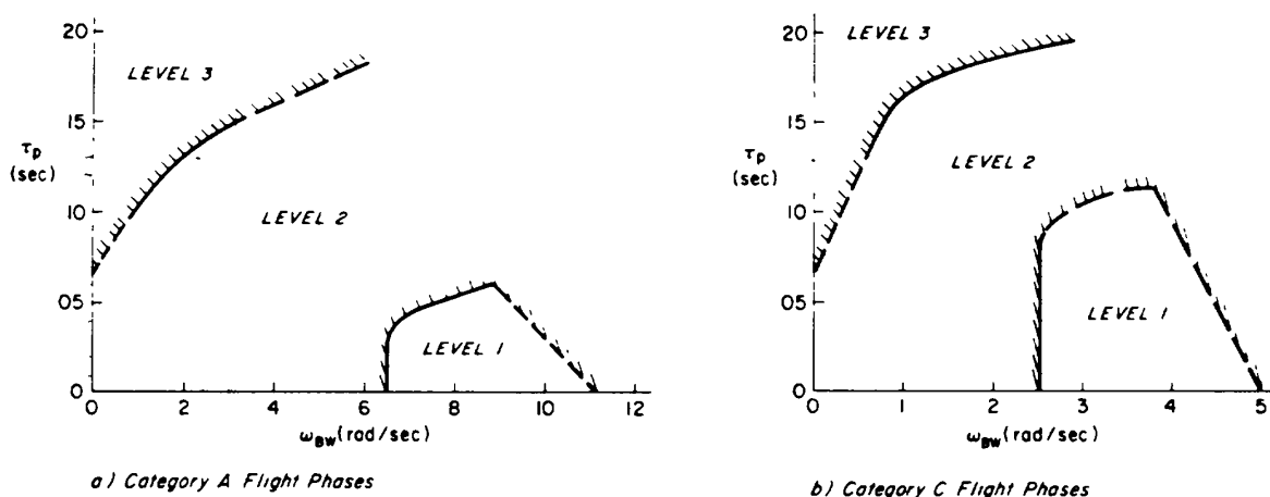
FIGURE 57. Bandwidth requirements.
