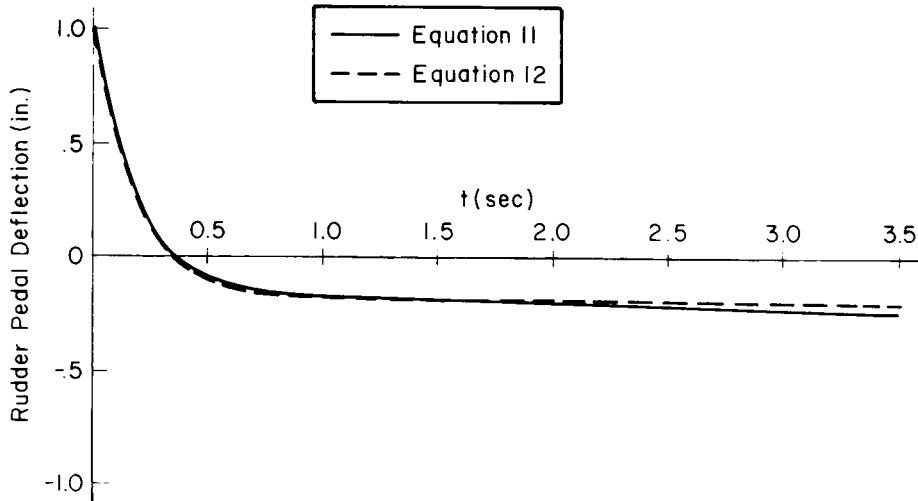
FIGURE 250. Effect of removing high-frequency roots from numerators.
