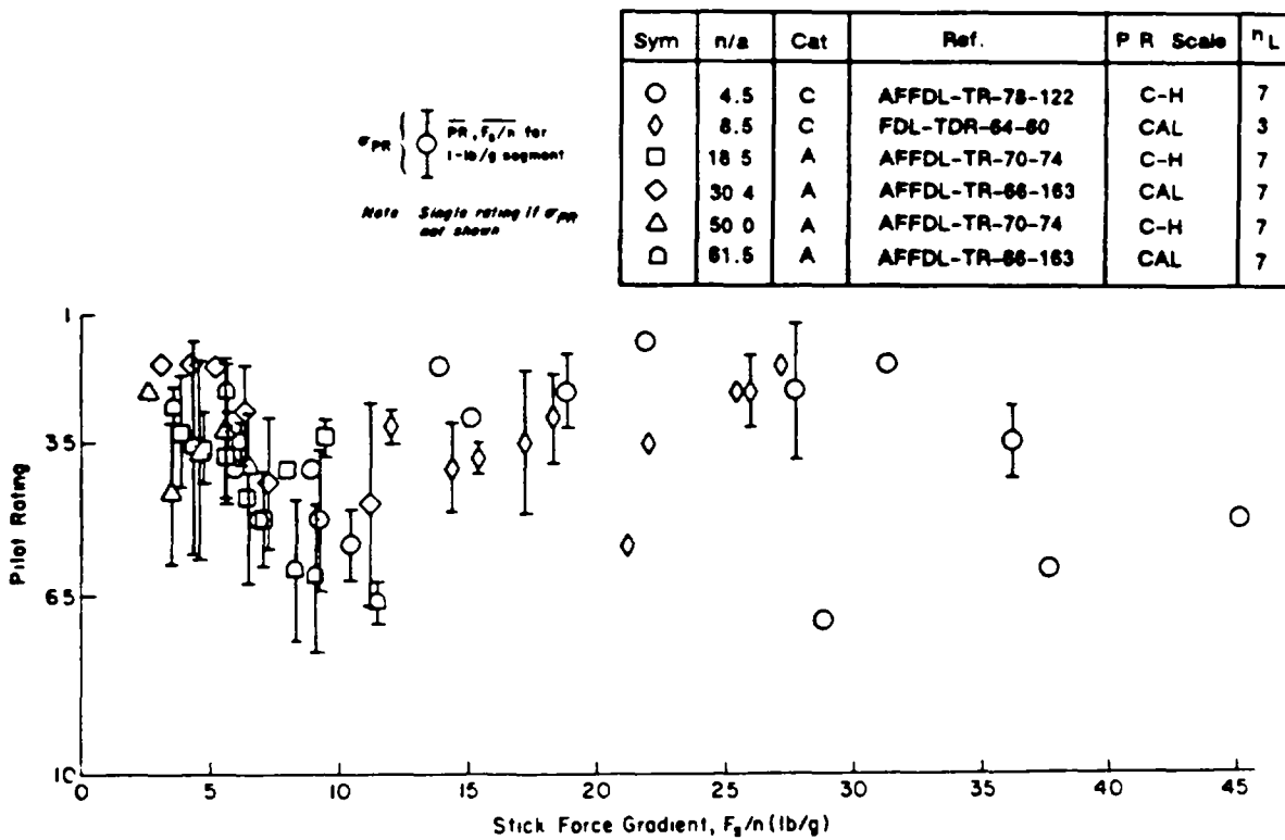
FIGURE 109. Average pilot ratings for 1-lb/g segments of F_s/n .
