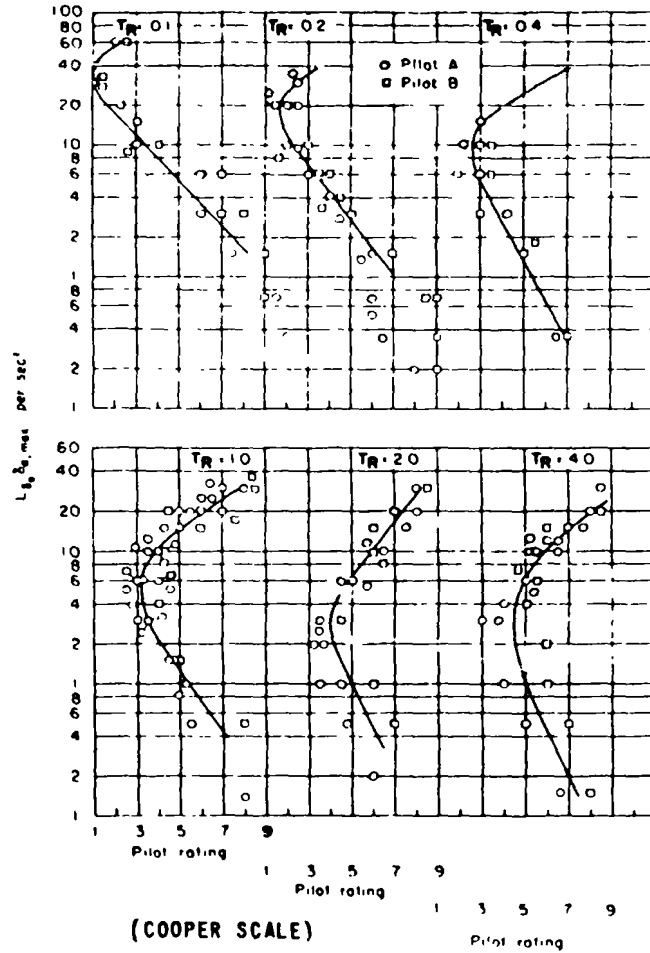
FIGURE 138. Variation of pilot opinion with L_{\delta_a} \delta_{a_{max}} for constant values of T_R as obtained from the stationary flight simulator (from NASA Memo 1-29-59A).
