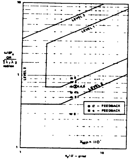
b) Canard, x_{mp} = 110 ft
