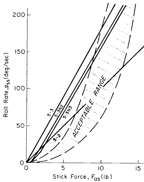
FIGURE 202. Roll gradients for LATHOS configurations 5-2 and 5-3 ( T_R = 0.15 sec) compared with acceptable range from figure 194.
