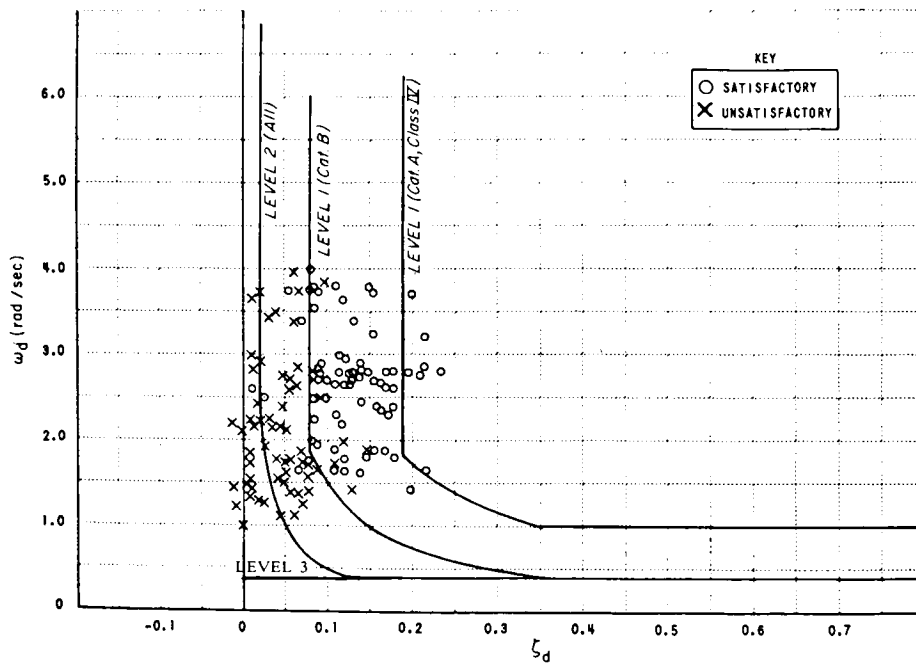
FIGURE 209. Dutch roll data (from Cornell Aero Lab Rpt TB-574-F-3).
