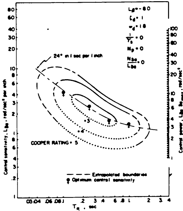
FIGURE 134. Lateral control boundaries (from Princeton Univ Rpt 727).
