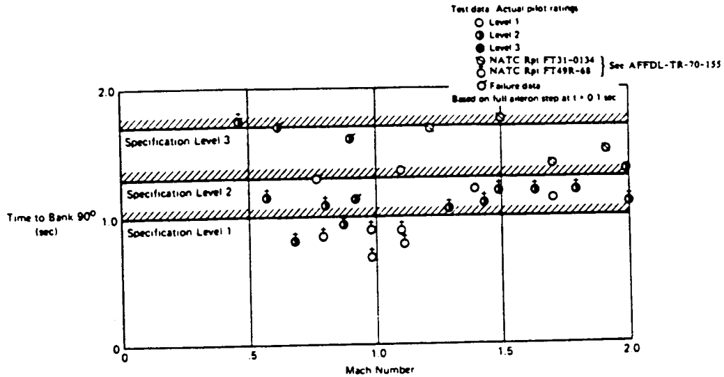
a) Time to Bank 90 deg
