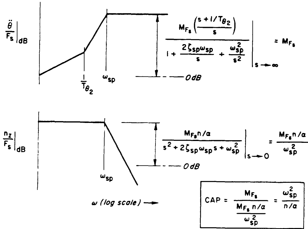
FIGURE 20. Definition of CAP from frequency response asymptotes.
