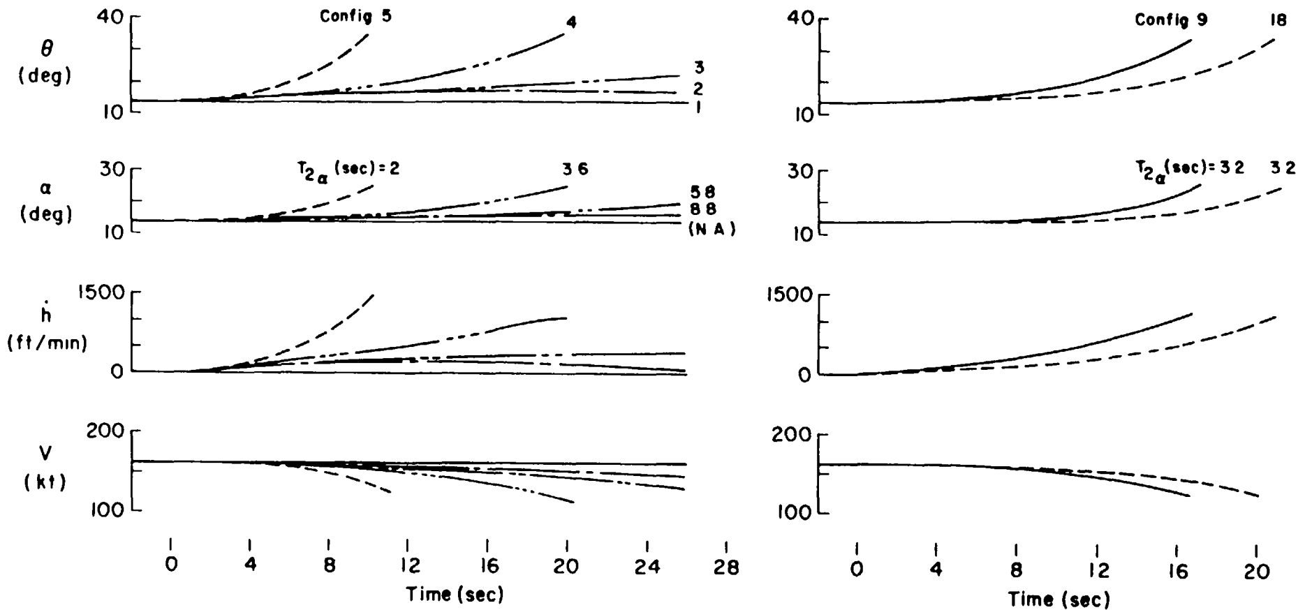
a) Comparison of Linear C_m(\alpha) Configurations 1-5
