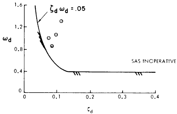
FIGURE 227. Lateral directional damping for some Class III airplanes (from AFFDL-TR-78-171).
