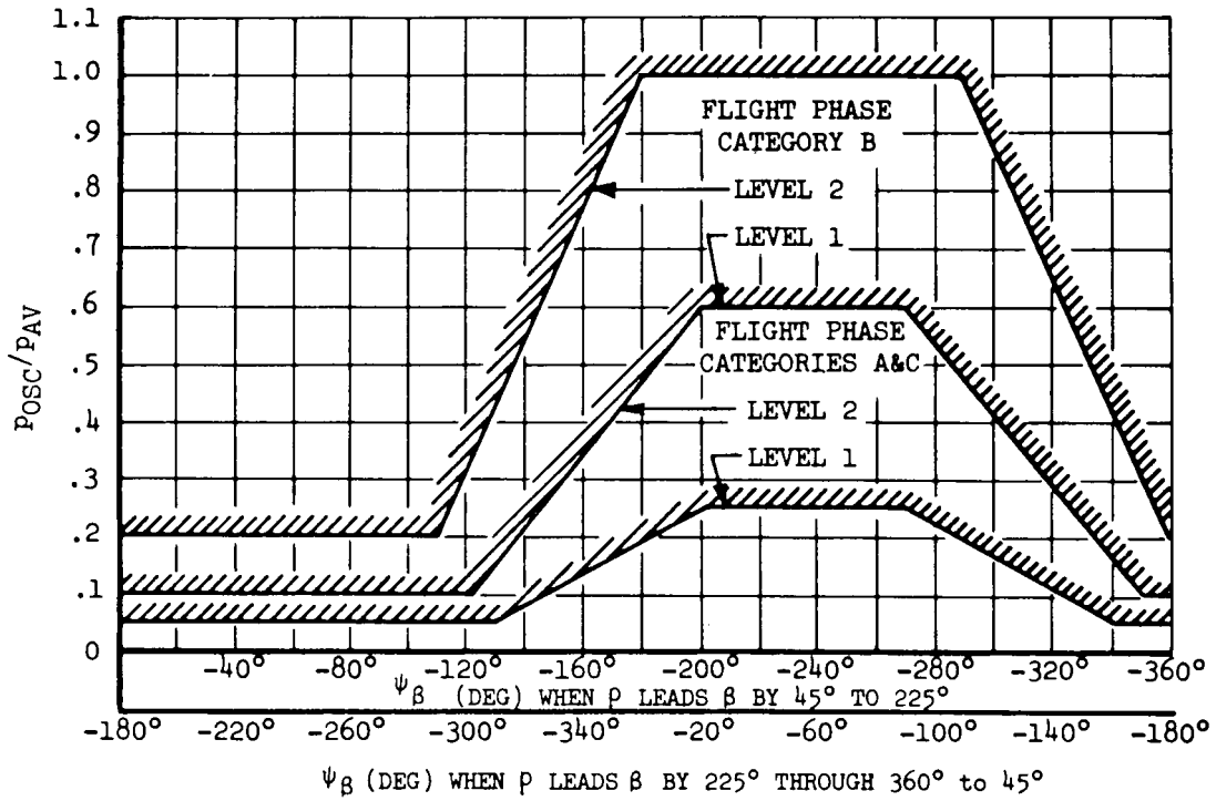
FIGURE 156. Roll rate oscillation limitations.
