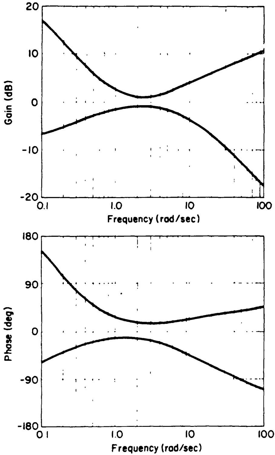
FIGURE 15. Envelopes of maximum unnoticeable added dynamics (AFWAL-TR-82-3064).
