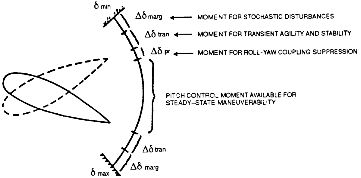
FIGURE 11. Control margin requirements.
