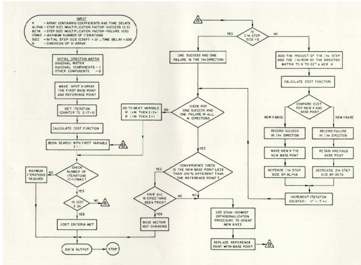
FIGURE 272. Flow Chart for a modified Rosenbrock search algorithm.
