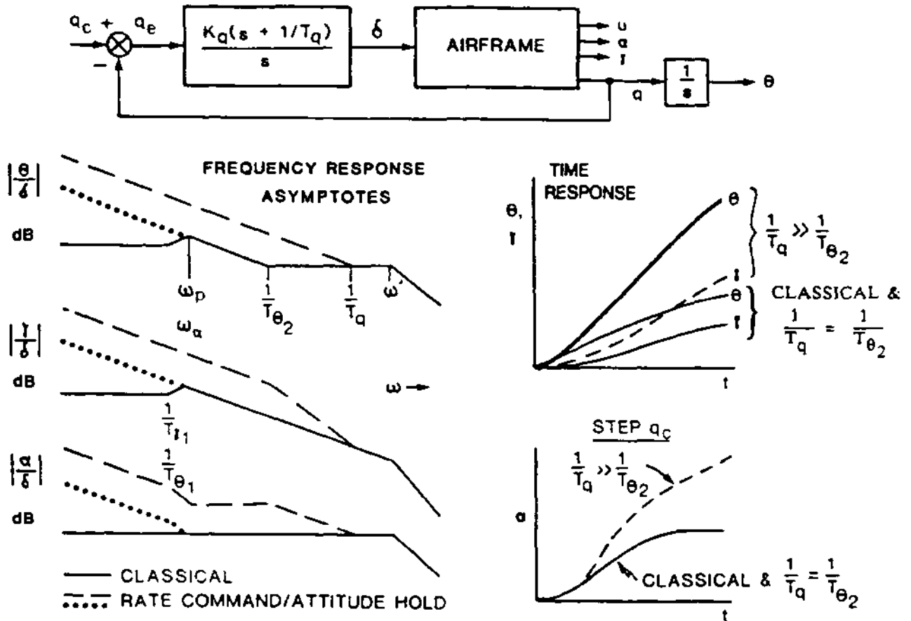
FIGURE 87. Frequency and time response comparison.
