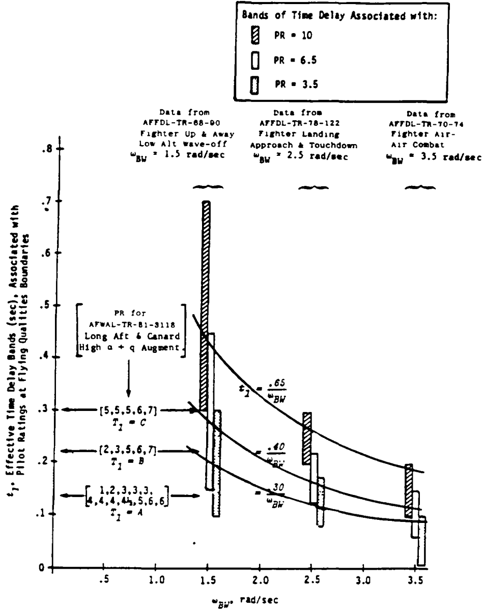
FIGURE 41. Time delay bands associated with flying qualities boundaries vs bandwidth, AFWAL-TR-81-3118.
