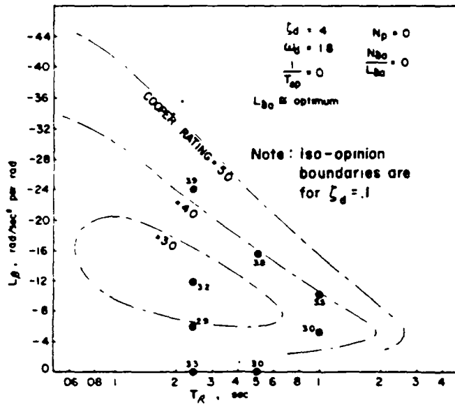
FIGURE 136. Lateral flying qualities boundaries ( L_{\beta} vs. T_R , \zeta_d = 0.4 ) (from Princeton Univ Rpt 727).
