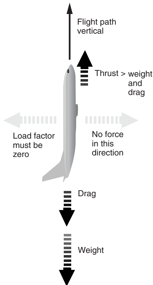
Figure 13a Airplane Vertical With Forces Balanced
