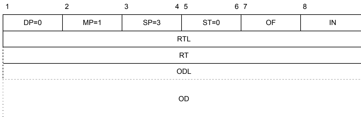
Figure 5-19. ROUTE packet
