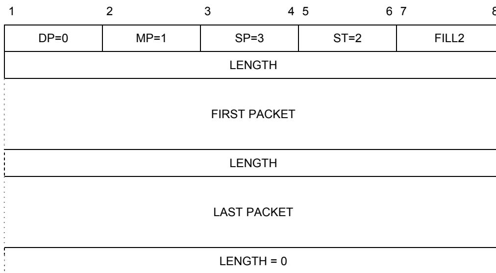
Figure 5-20. MULTIPLEX packet
